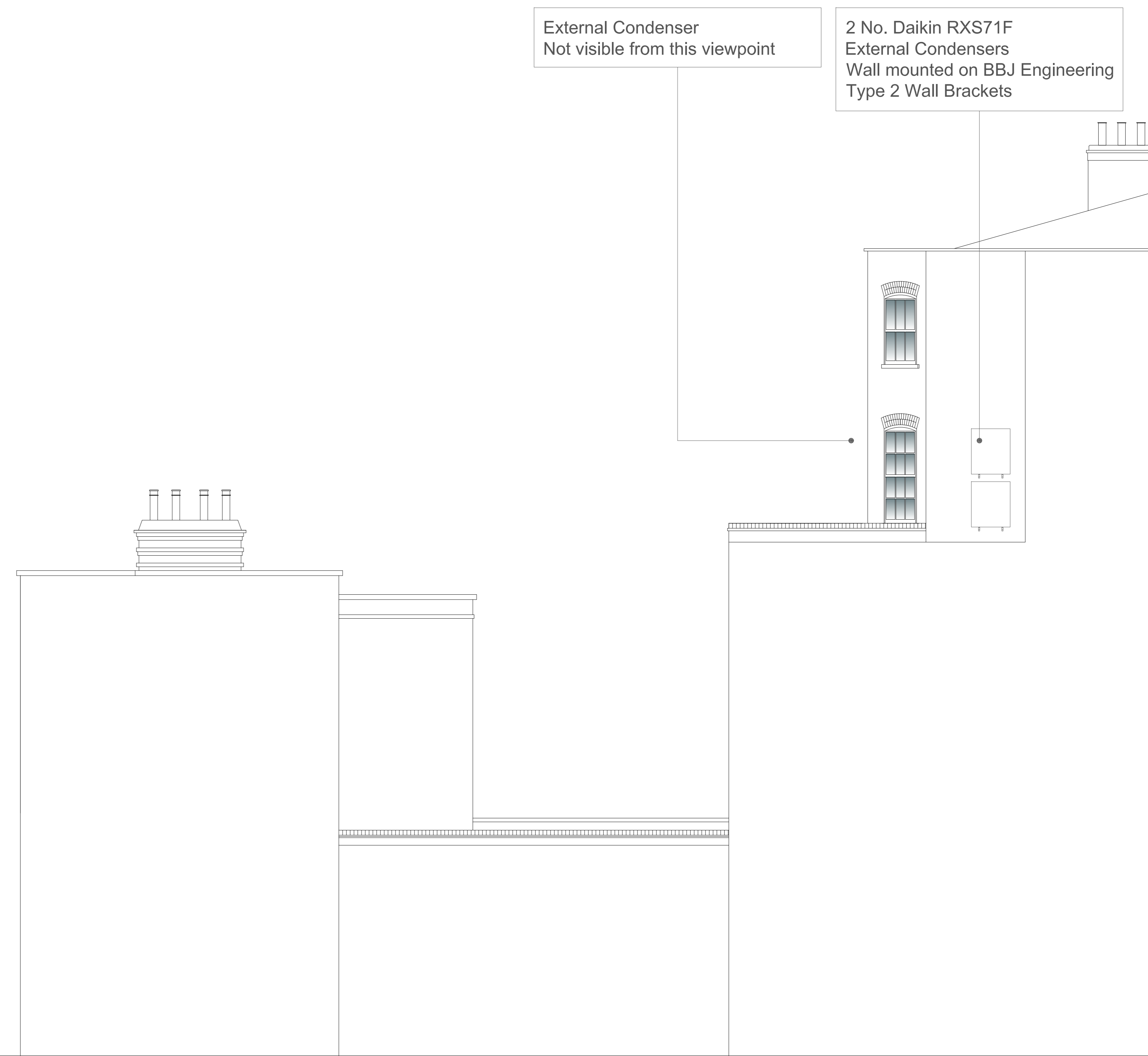
Proposed Side Elevation (SE)
