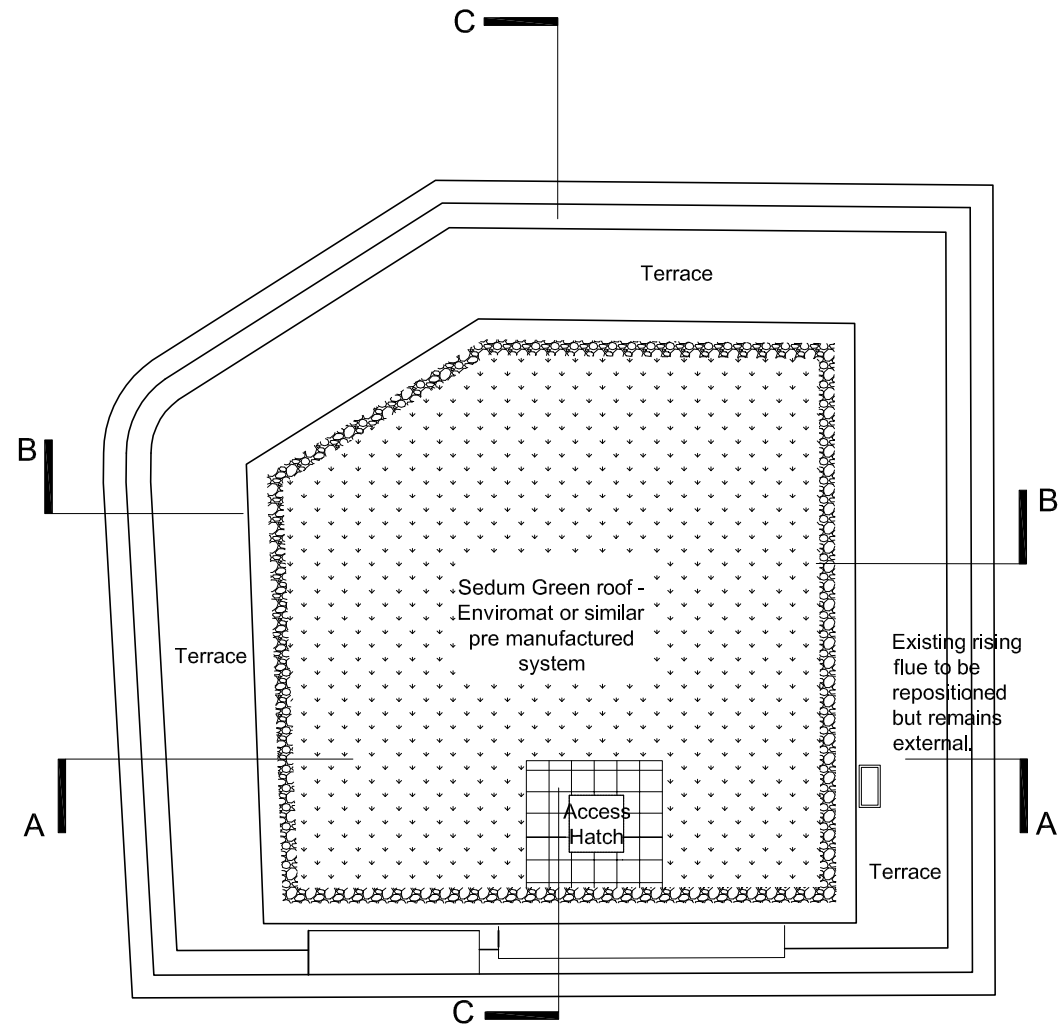
ROOF PLAN
