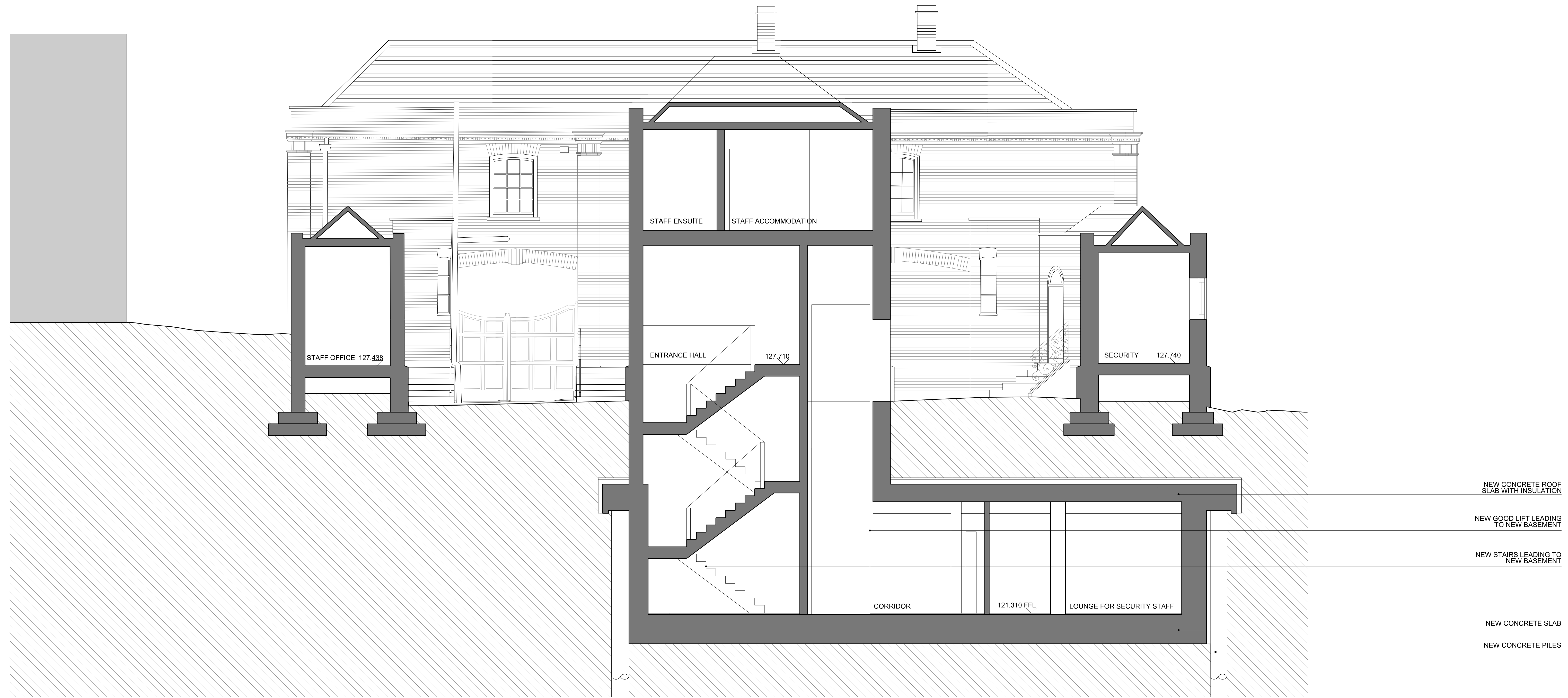
01 SECTION QQ 1:50 @ A0
