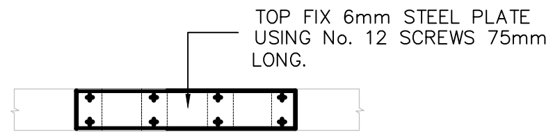
PLAN ON MULTI-NOTCH REPAIR
