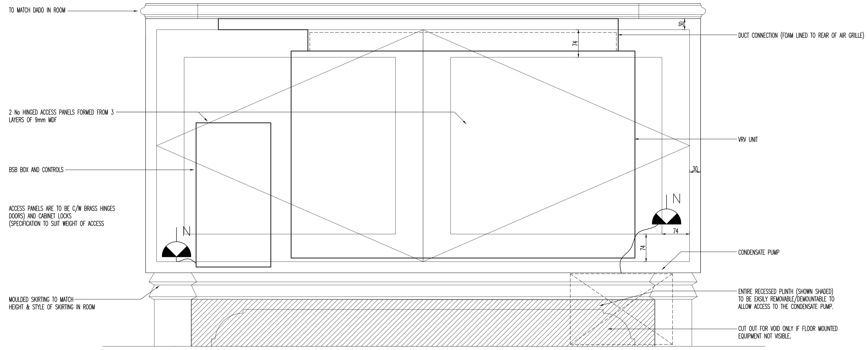
FRONT VIEW
