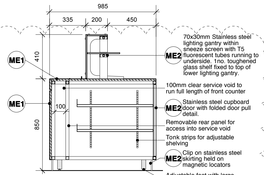
03 SECTION B - AMBIENT 1:20@ A3
