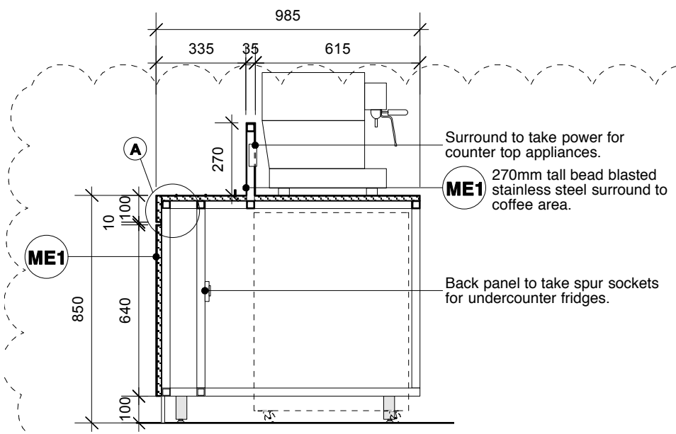
01 SECTION A - COFFEE 1:20@ A3
