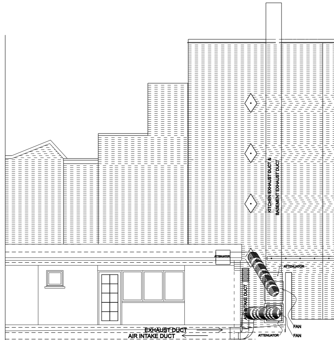
71 HAMPSTEAD HIGH STREET REAR EXTENSION
