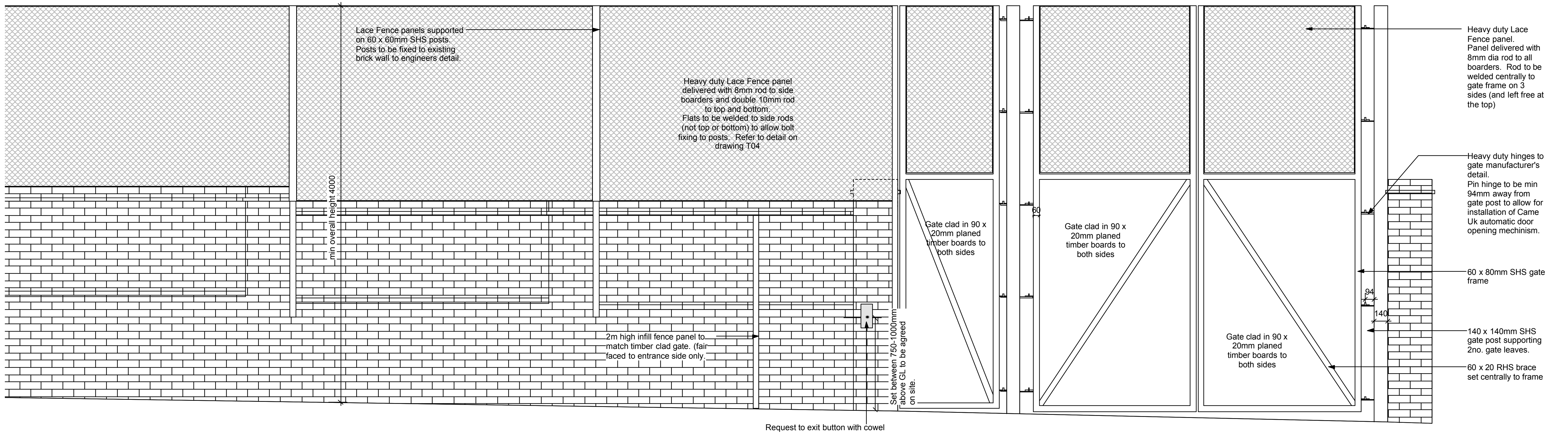
Elevation of Eastern Entrance Scale 1:20
