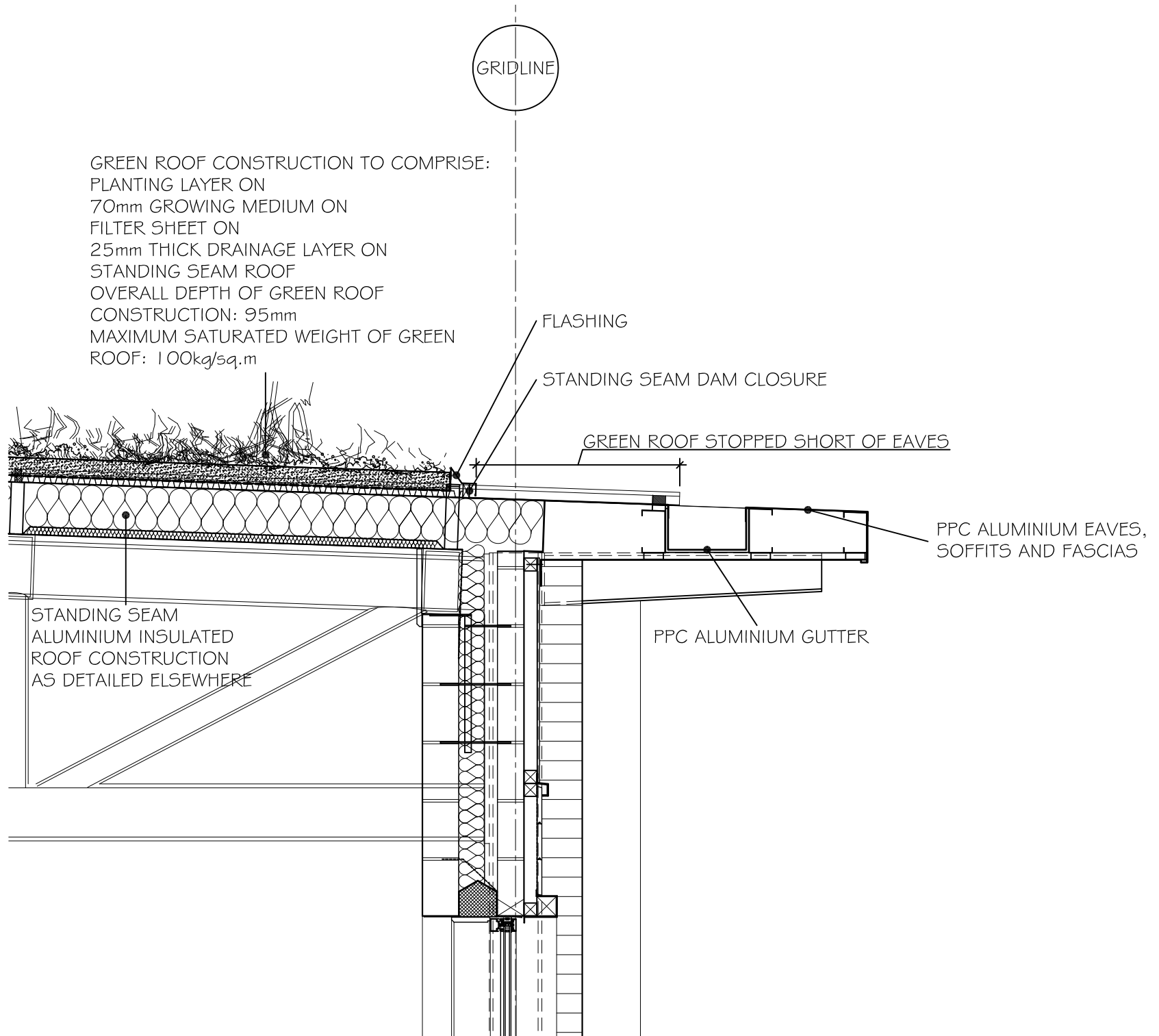
TYPICAL EAVES DETAIL SHOWING GREEN ROOF CONSTRUCTION 1:20
