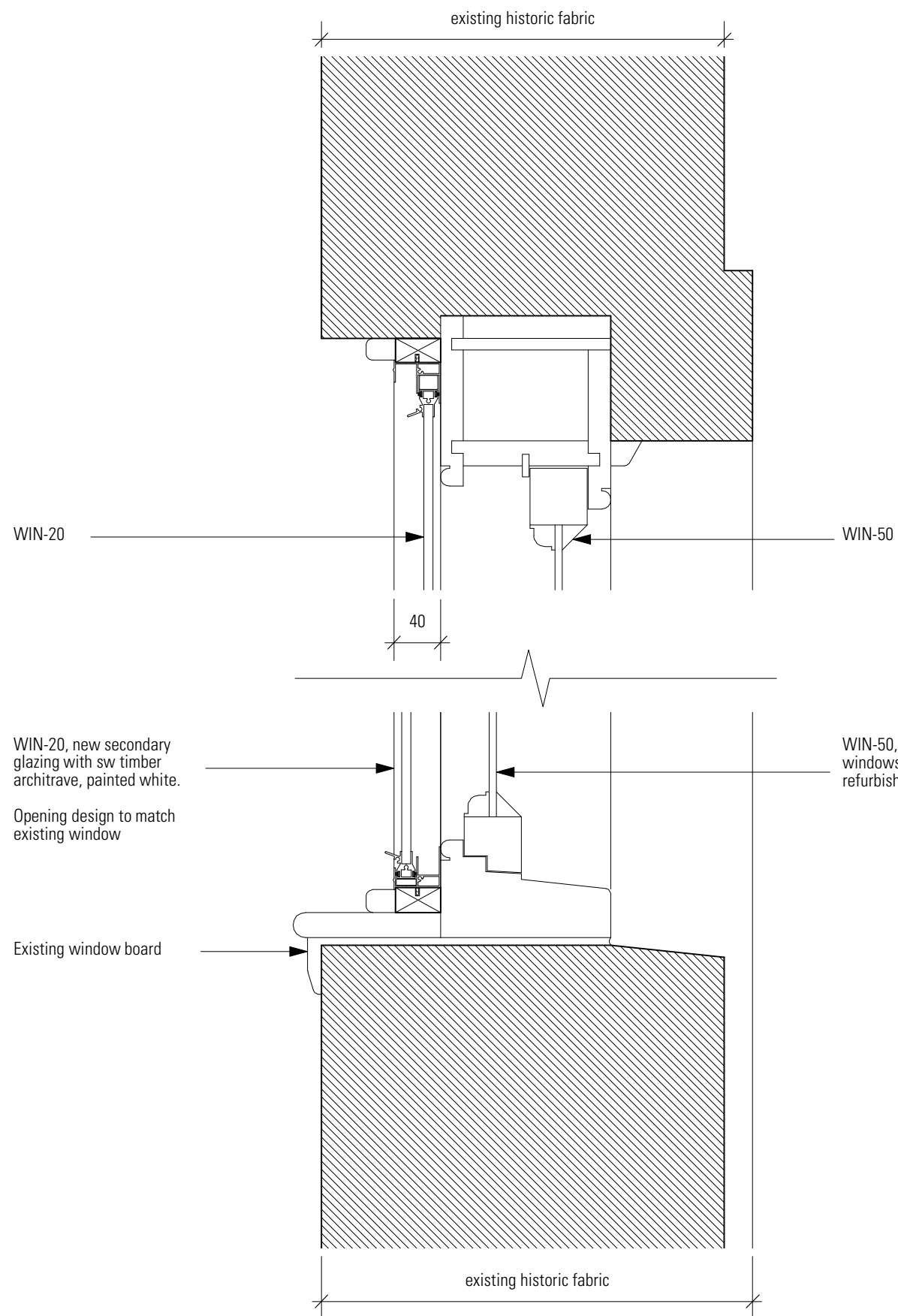
1 Typical Heritage Window Head & Cill Detail 1:5
