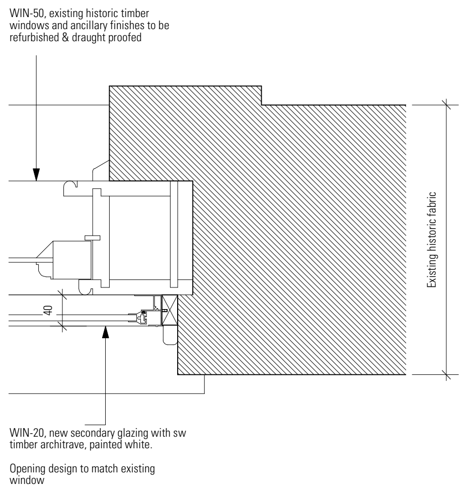
2 Typical Heritage Window Jamb Detail 1:5
