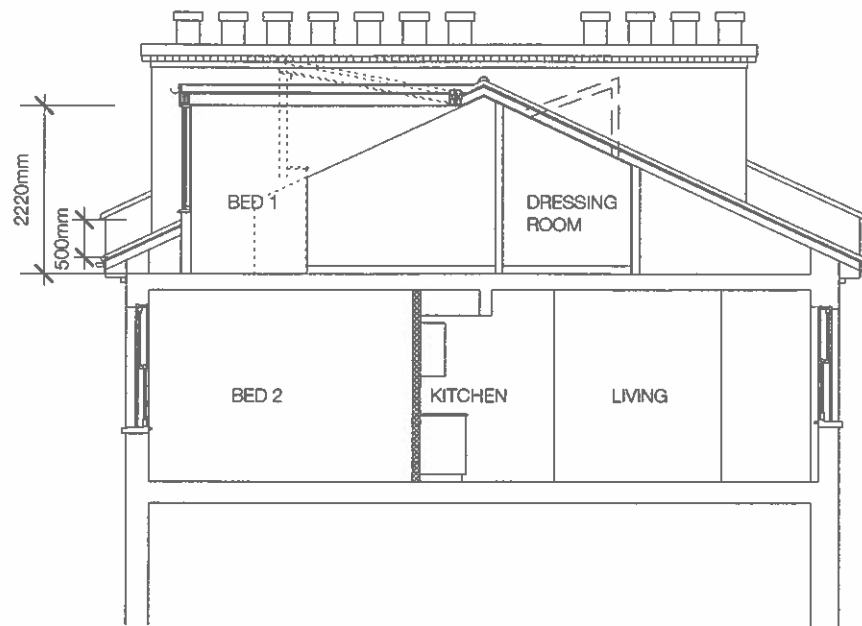
SECTION
