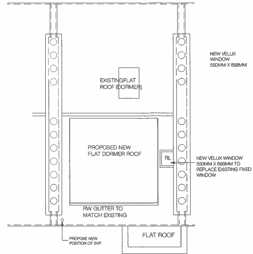
ROOF PLAN
