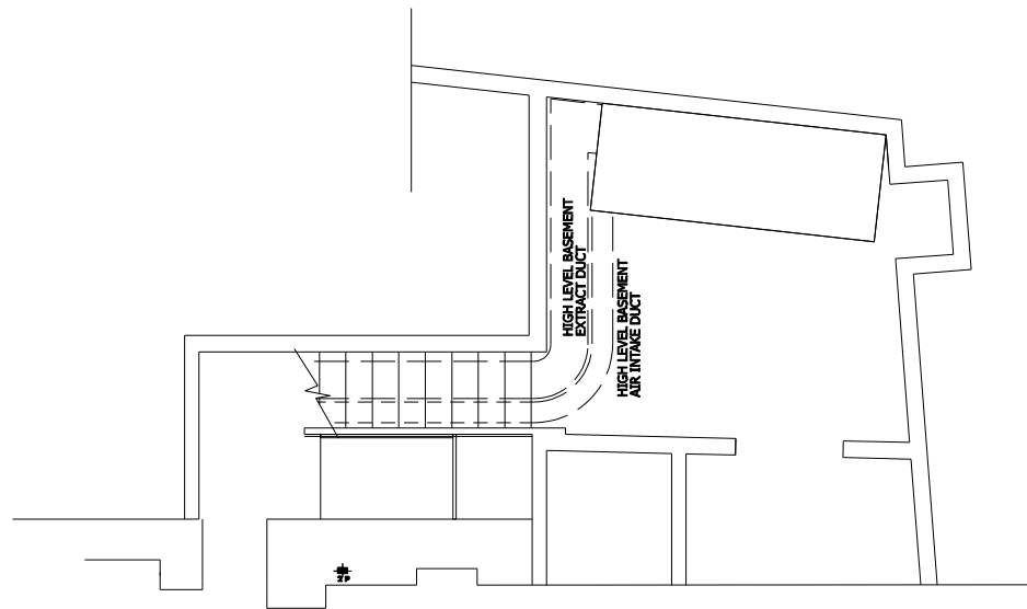
BASEMENT PLAN PROPOSED DUCT LAYOUT
