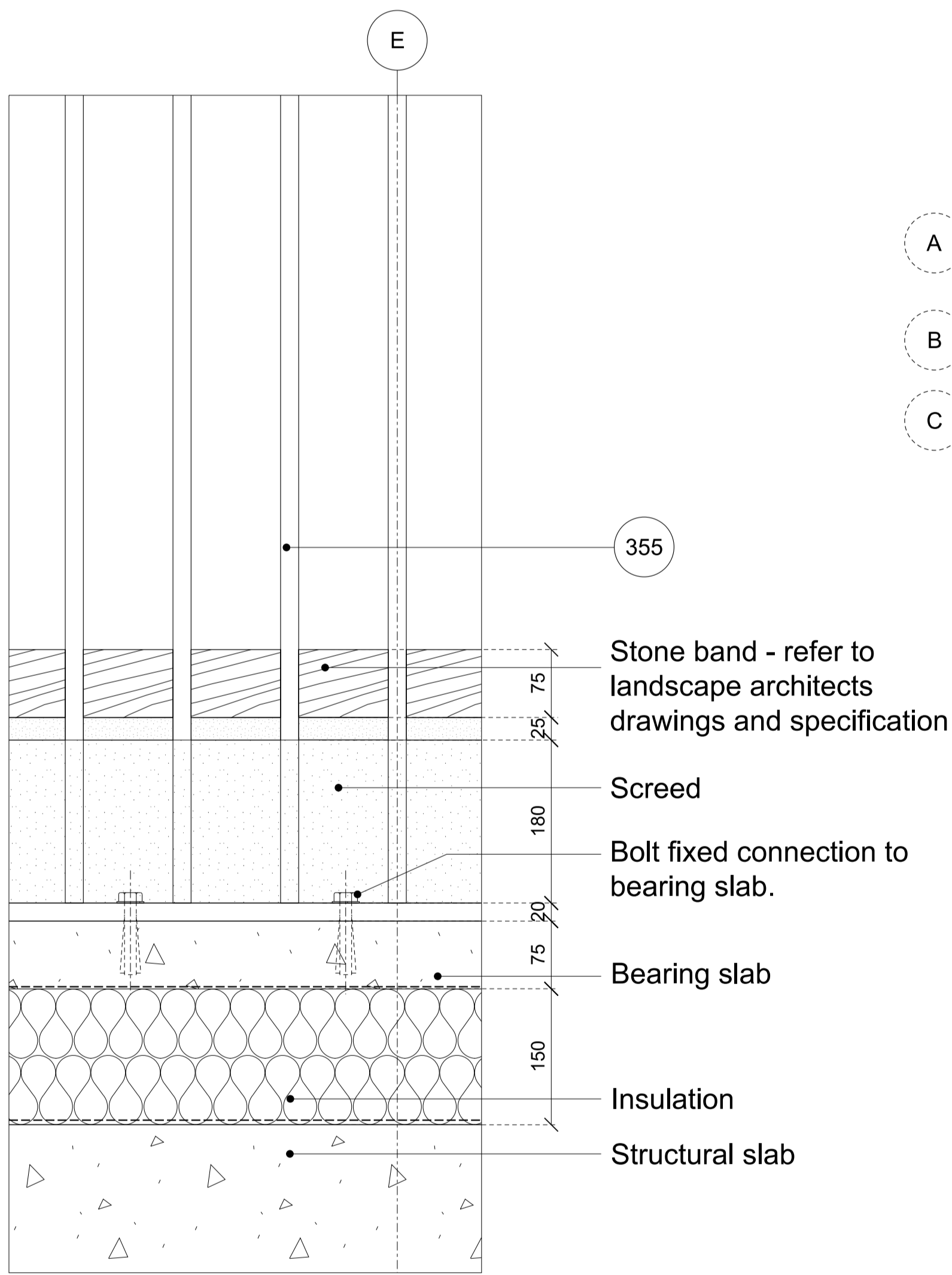
04 MONTAGUE PLACE RAILING 1:5
