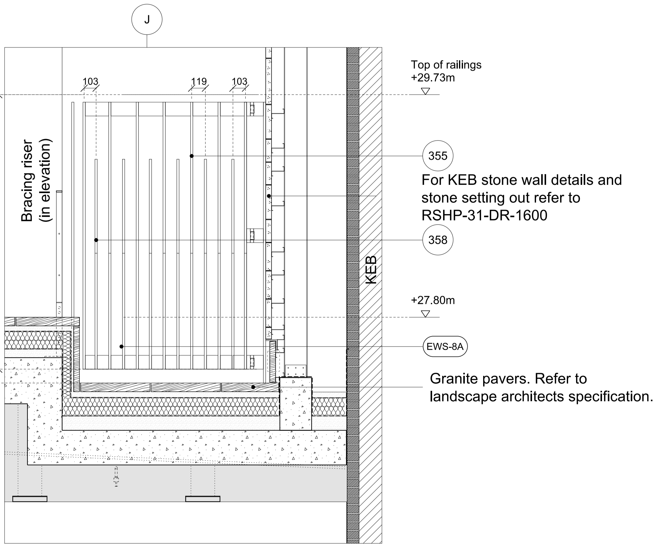
05 LONG SECTION - KEB WALL GATE 1:20
