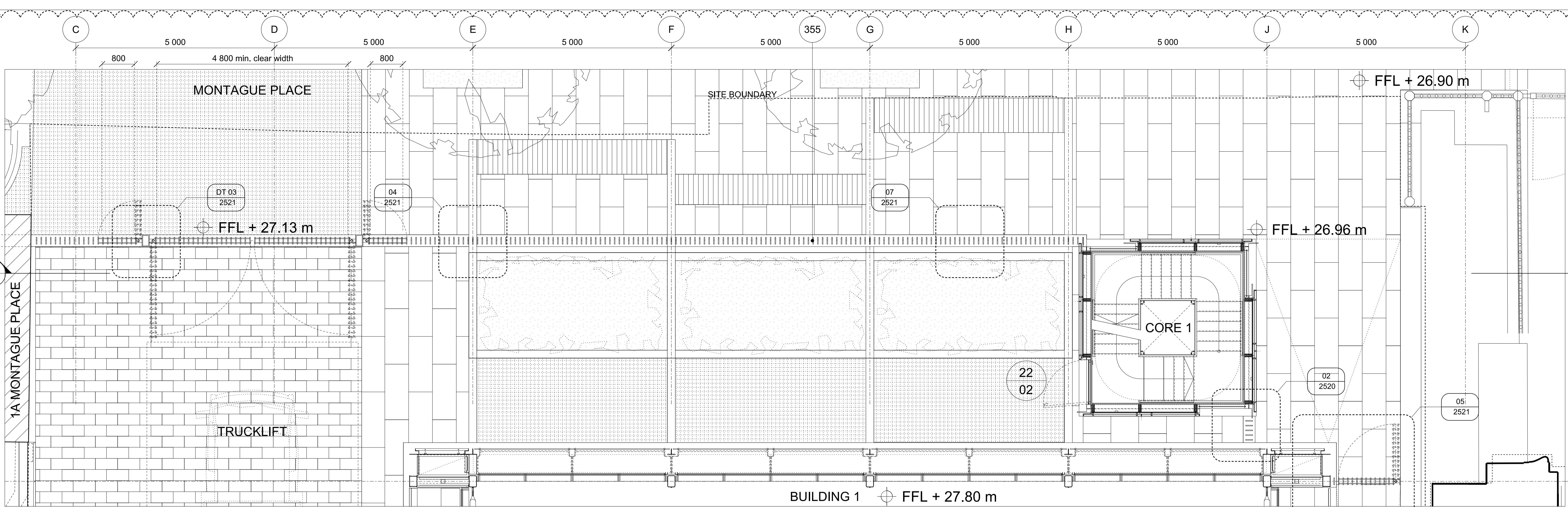
01 PLAN - RAILING TYPE BAL-106 1:50
