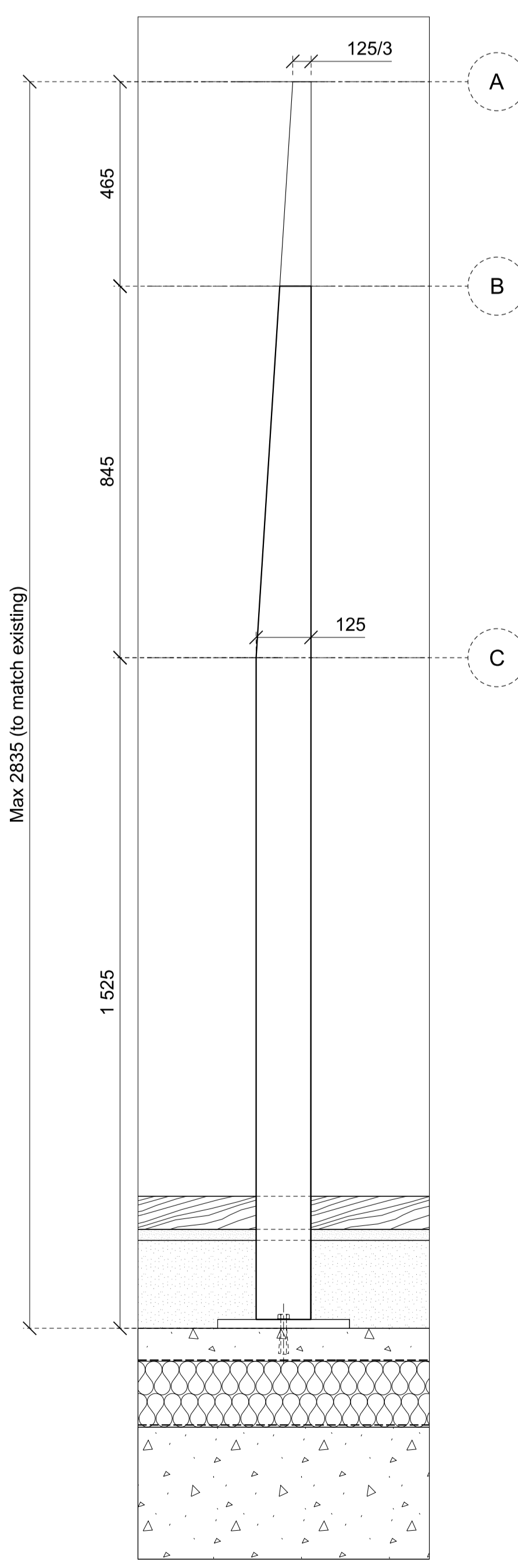
07 SHORT ELEVATION 1:10
