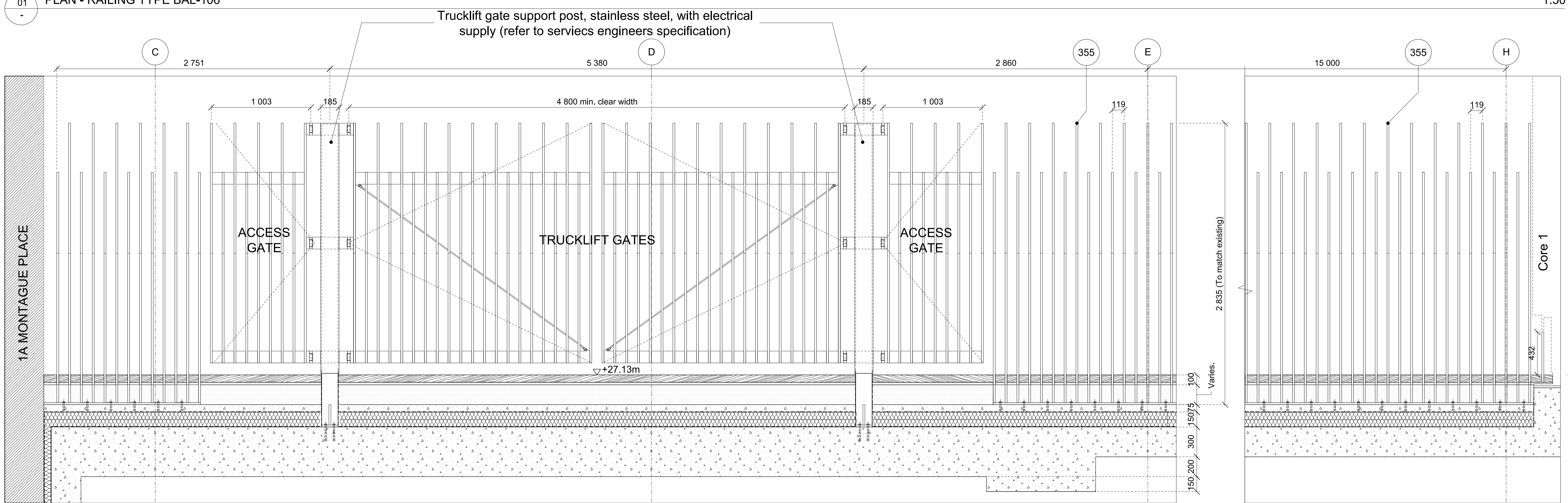
02 LONG SECTION - TRUCKLIFT GATES AND MONTAGUE PLACE RAILINGS 1:20
