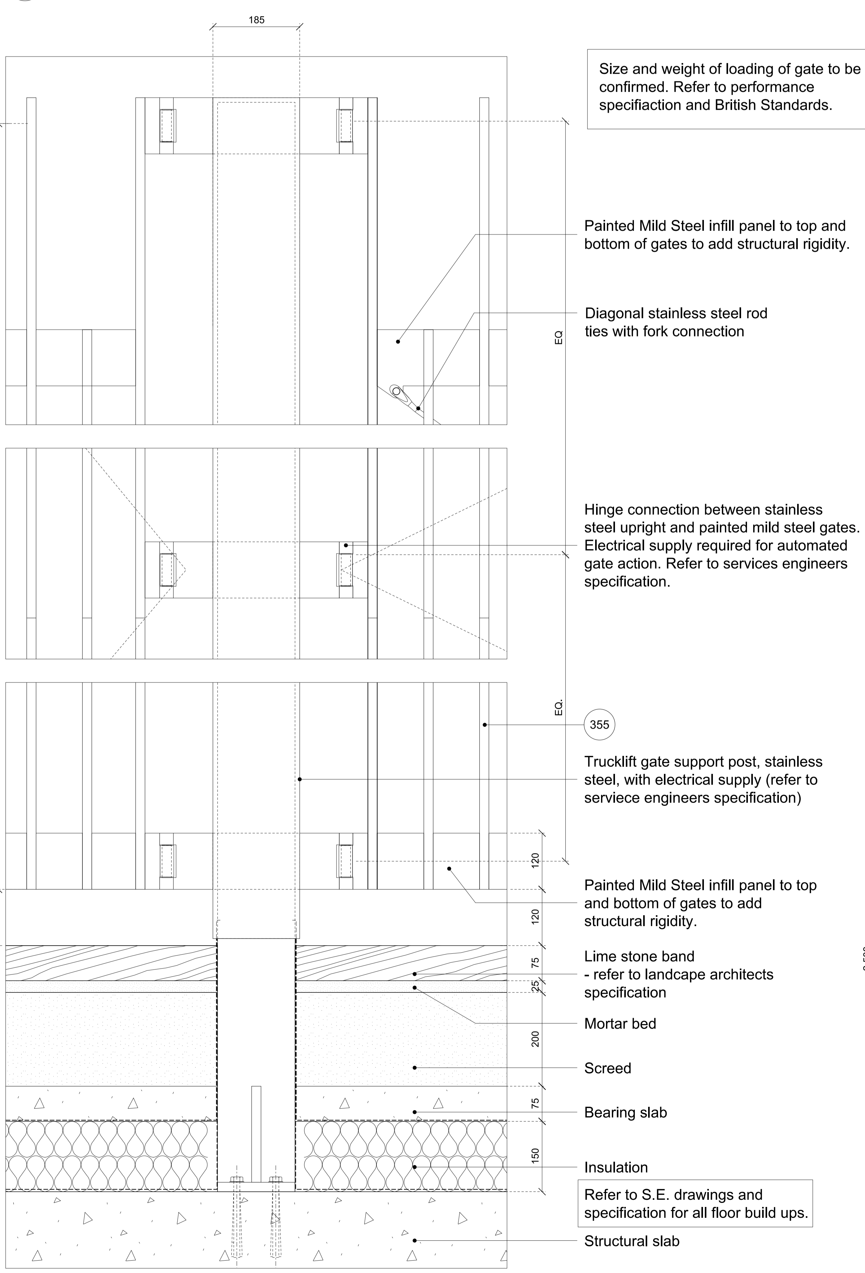
03 TRUCKLIFT GATE - POST SUPPORT 1:5
