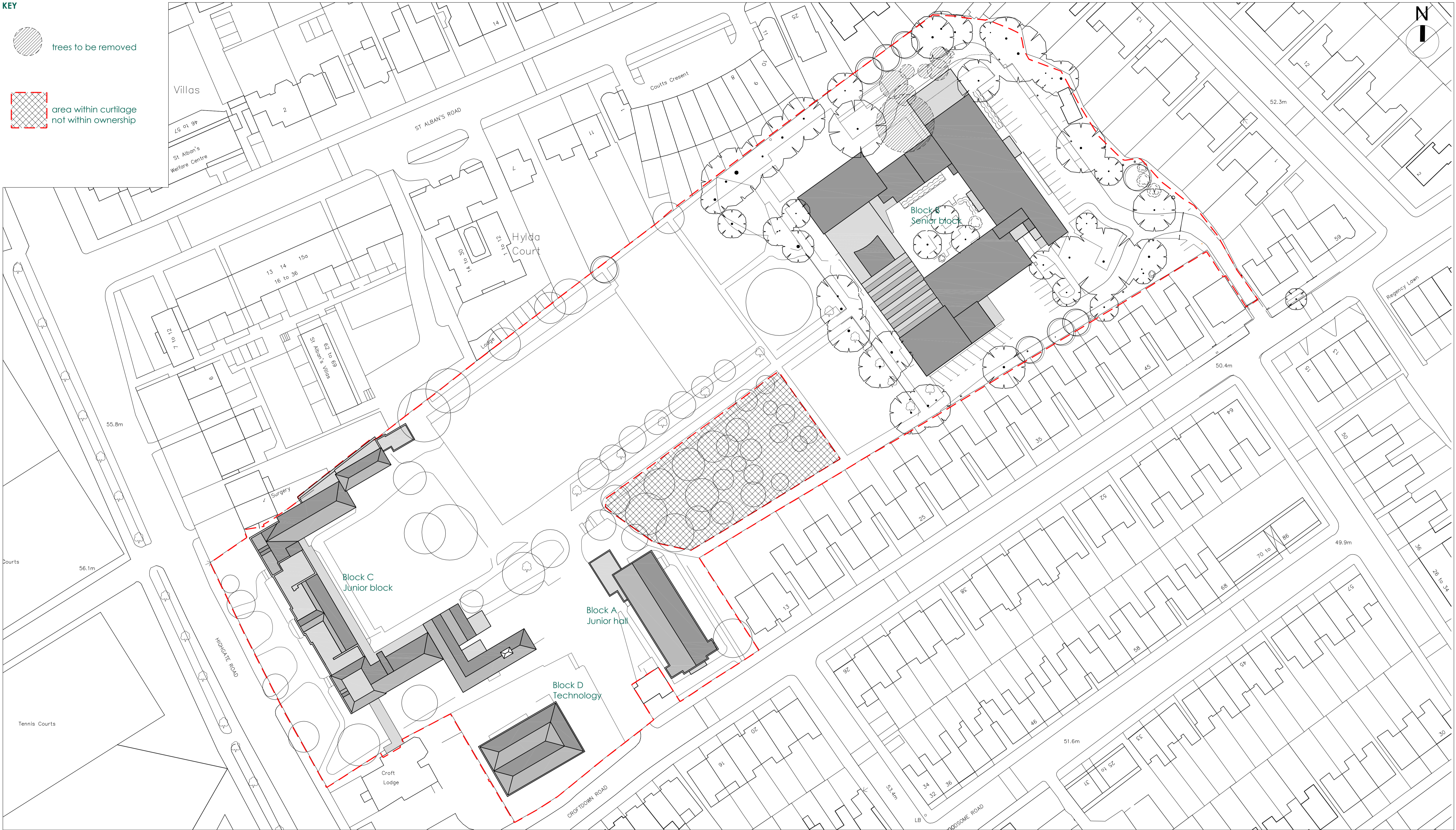
Existing site plan 1:500
