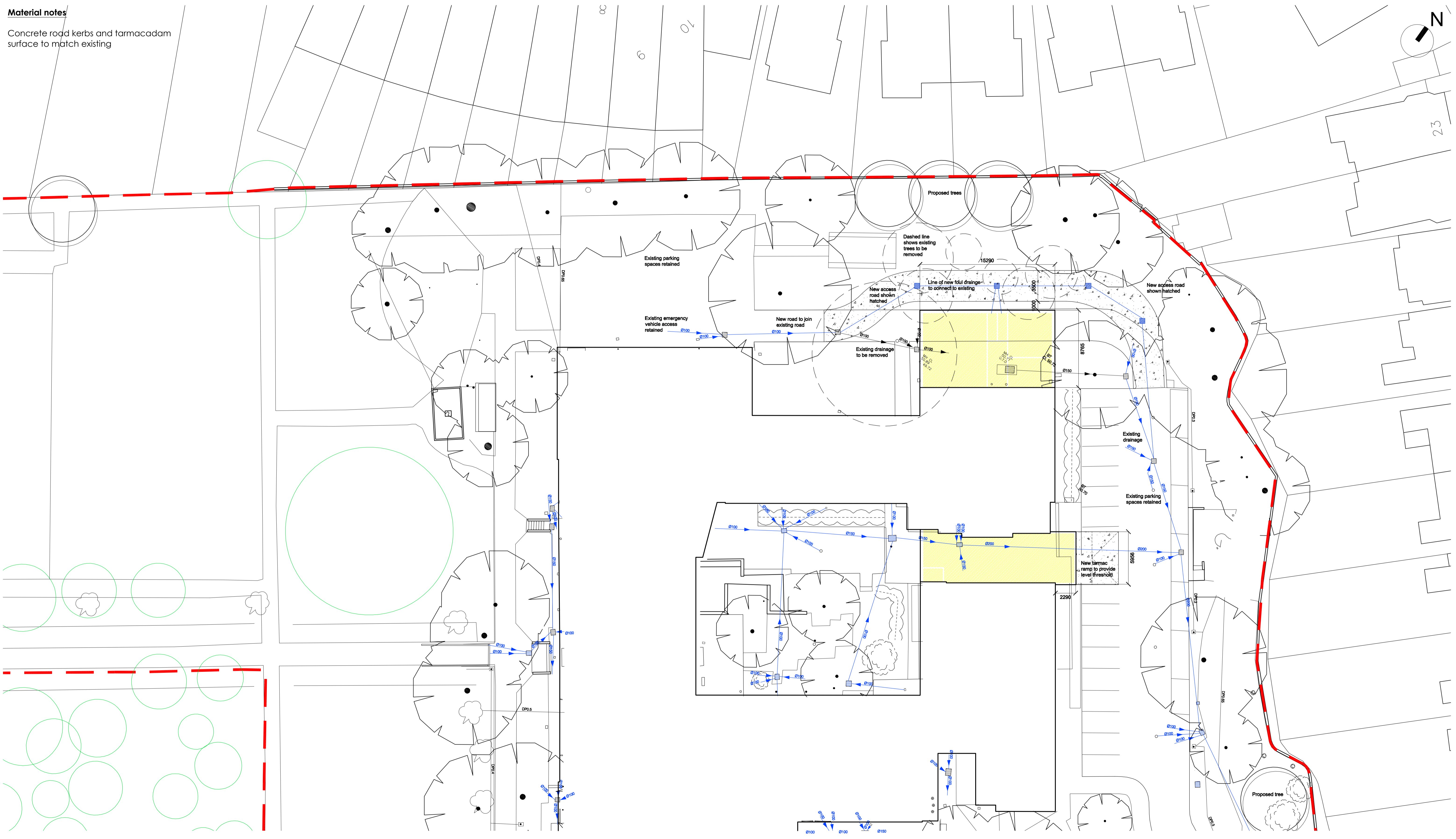
Proposed external works plan
