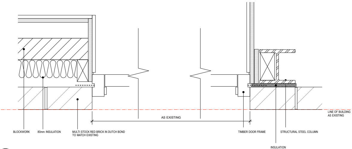
2 JAMB DETAILS 1:10 @ A3
