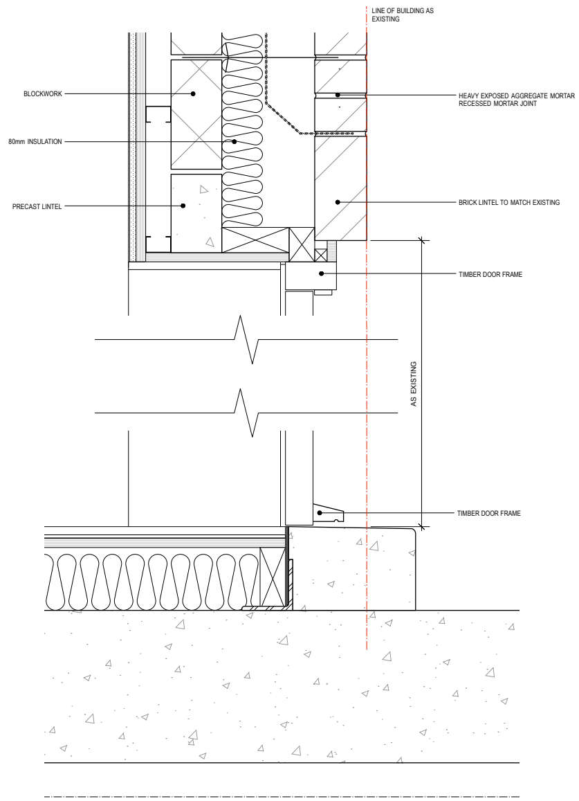
3 HEAD AND THRESHOLD DETAILS 1:10 @ A3
