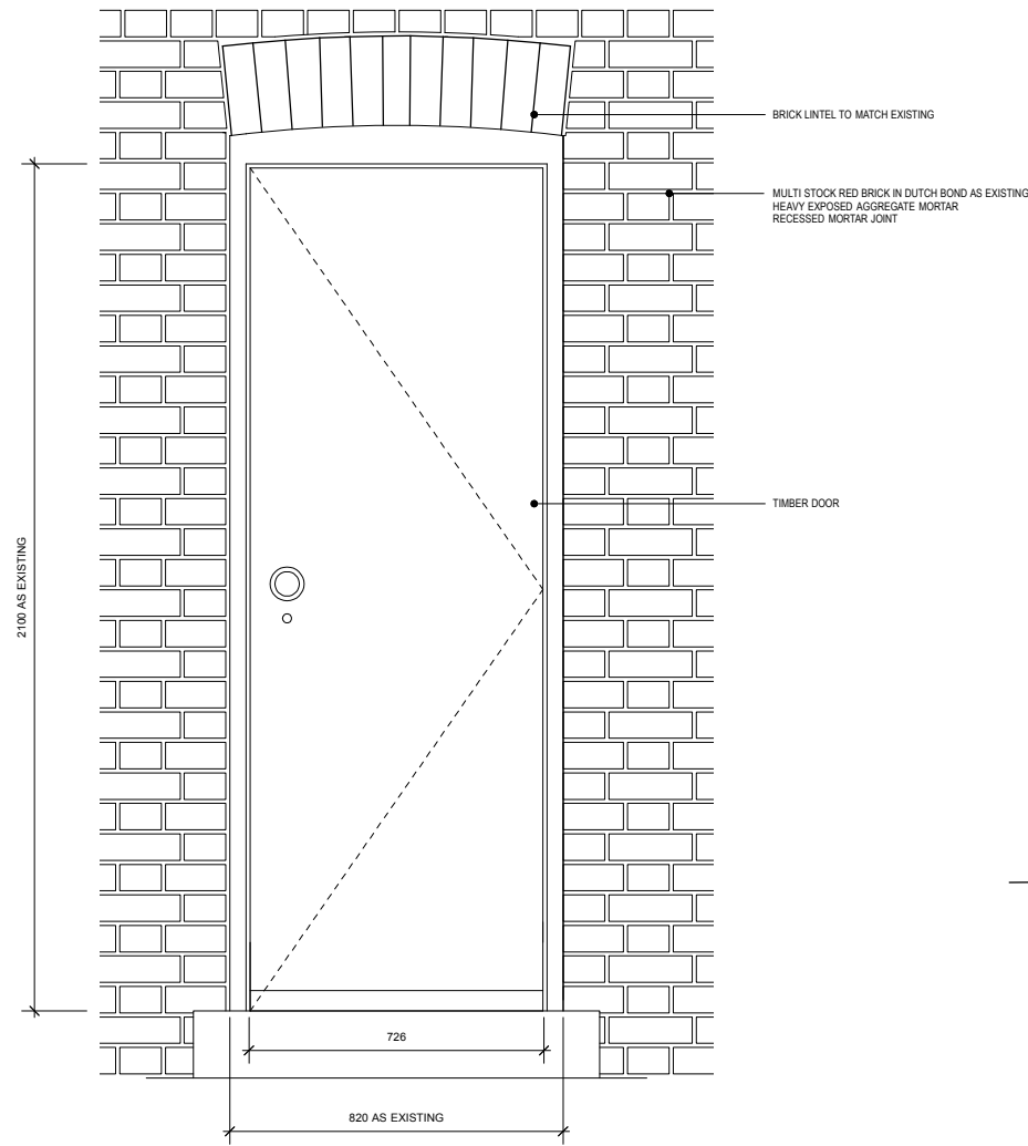
1 ELEVATION OF SIDE DOOR TO BUILDING A 1:20 @ A3
