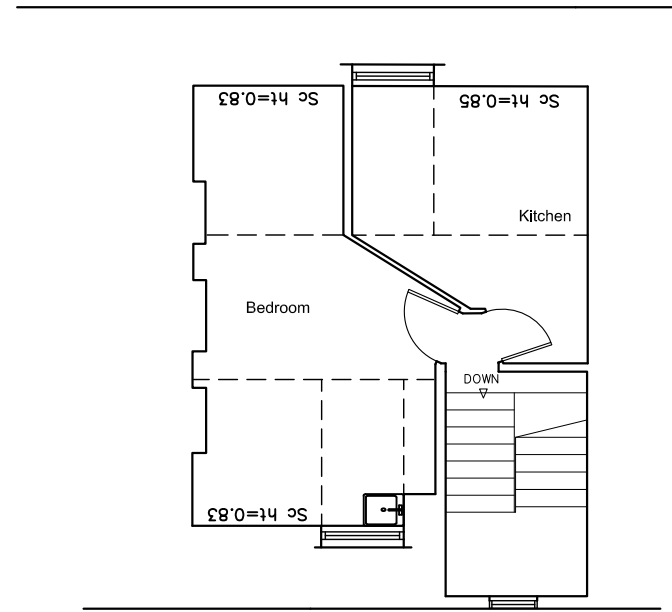
Existing Loft
