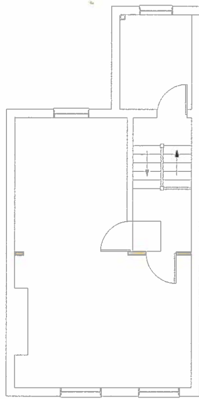
EXISTING FIRST FLOOR
