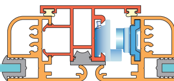
MEETING STILE (DOUBLE CASEMENT)
