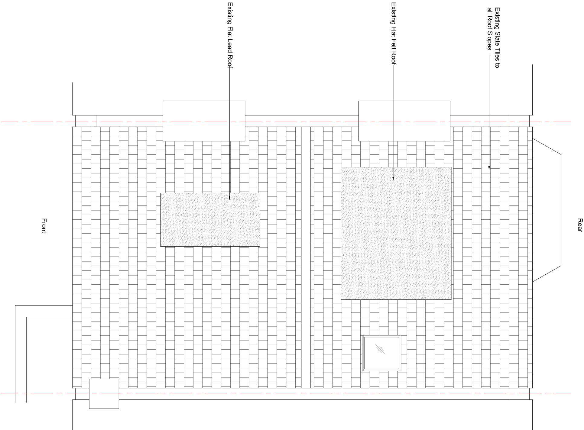
Existing Roof Plan Scale 1:50
