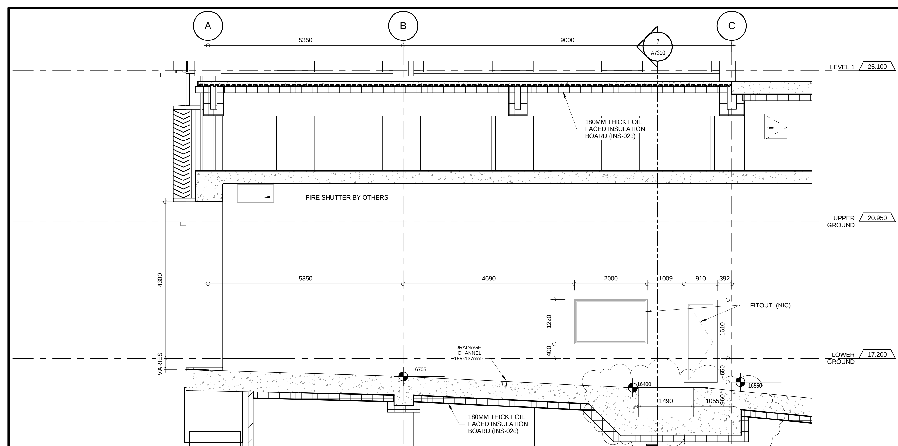
SECTION THRU VEHICLE RAMP 3 1 : 50 A4021
