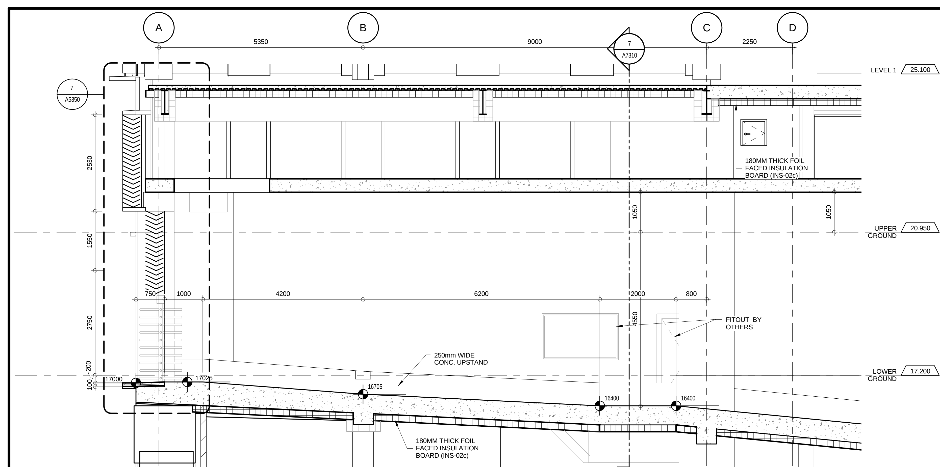
SECTION THRU PEDESTRIAN RAMP 1 : 50 9 A4021
