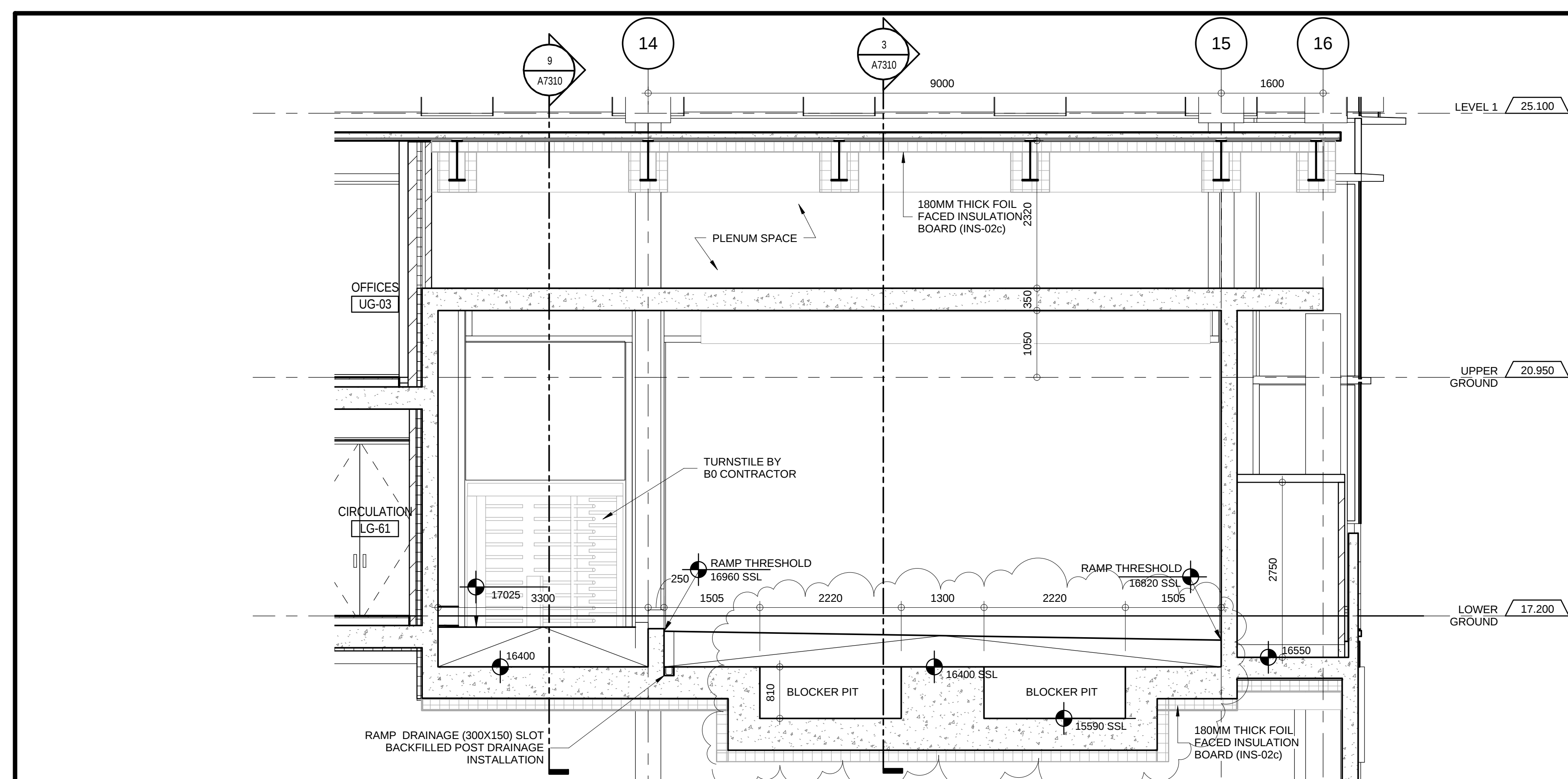
SECTION THRU BLOCKERS 7 1 : 50 A4102
