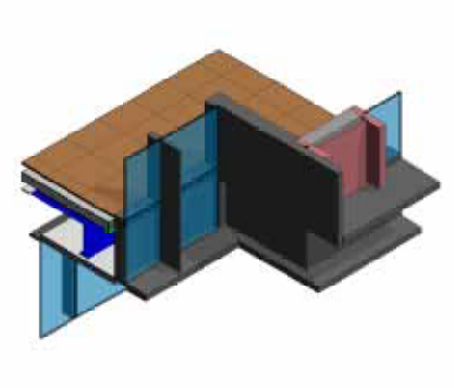
CLADDING TYPE T1 FULL HEIGHT DOUBLE GLAZED CURTAIN WALL SYSTEM WITH VERTICAL EXTER- NAL ALUMINIUM FINIS.
