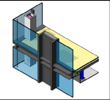
CLADDING TYPE T3 DOUBLE GLAZED CURTAIN WALL SYSTEM WITH VERTICAL ALUMINIUM SPANDREL PAN- EL AND FEATURE FINS AND CHANNEL.
