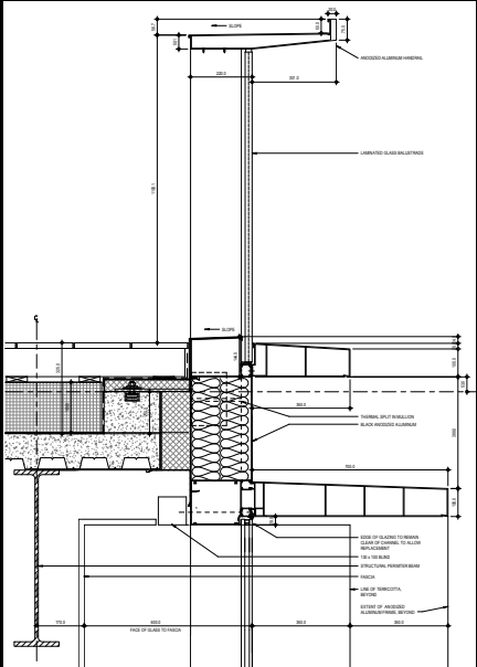
TYPICAL BALUSTRADE DETAIL
