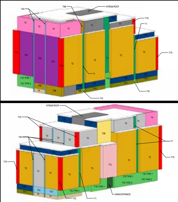
CLADDING TYPE T1G TOP PART: EXTERNALLY VENTILATED DOUBLE SKIN CURTAIN WALL. OUTER LEAF SINGLE GLAZED. INTERSTITIAL BLIND. BOTTOM PART: SPANDREL PANEL WITH SHADOW BOX.
