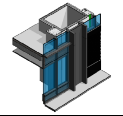
CLADDING TYPE T1G TOP PART: EXTERNALLY VENTILATED DOUBLE SKIN CURTAIN WALL. OUTER LEAF SINGLE GLAZED. INTERSTITIAL BLIND. BOTTOM PART: SPANDREL PANEL WITH SHADOW BOX.
