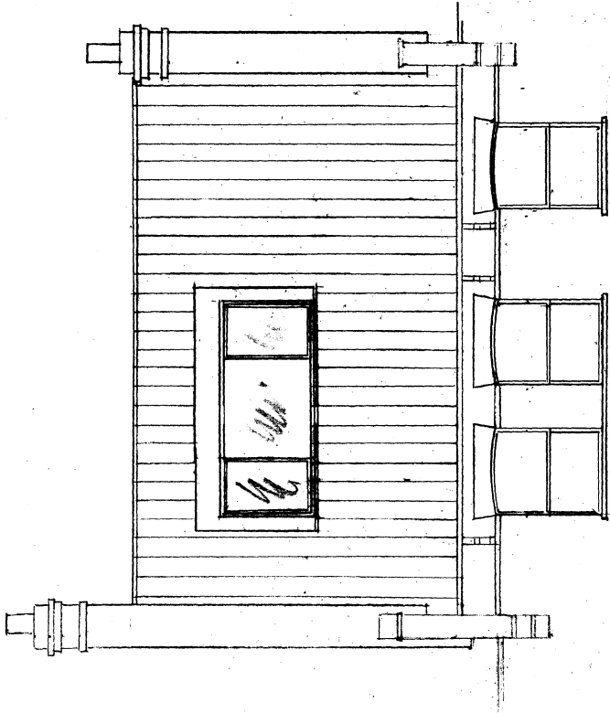
SOUTH - EAST ELEVATION
