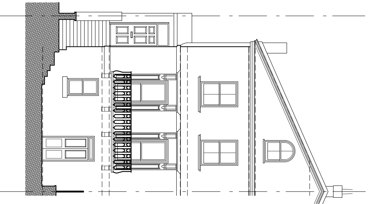
FRONT ELEVATION C-C - (AS EXISTING)
