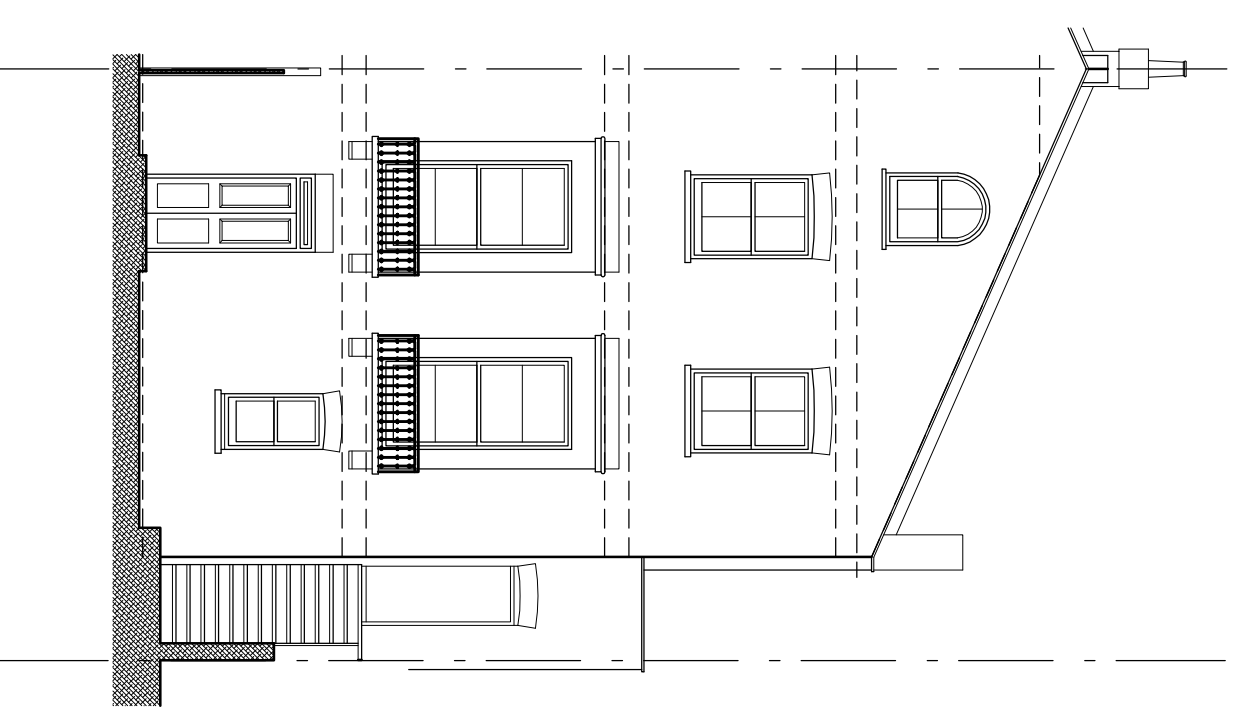
REAR ELEVATION D-D - (AS EXISTING)
