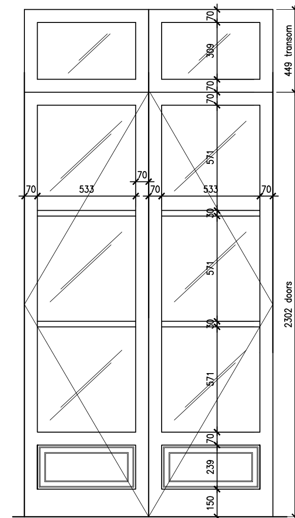
3 Proposed Terrace Door Scale: 1:20@ A3
