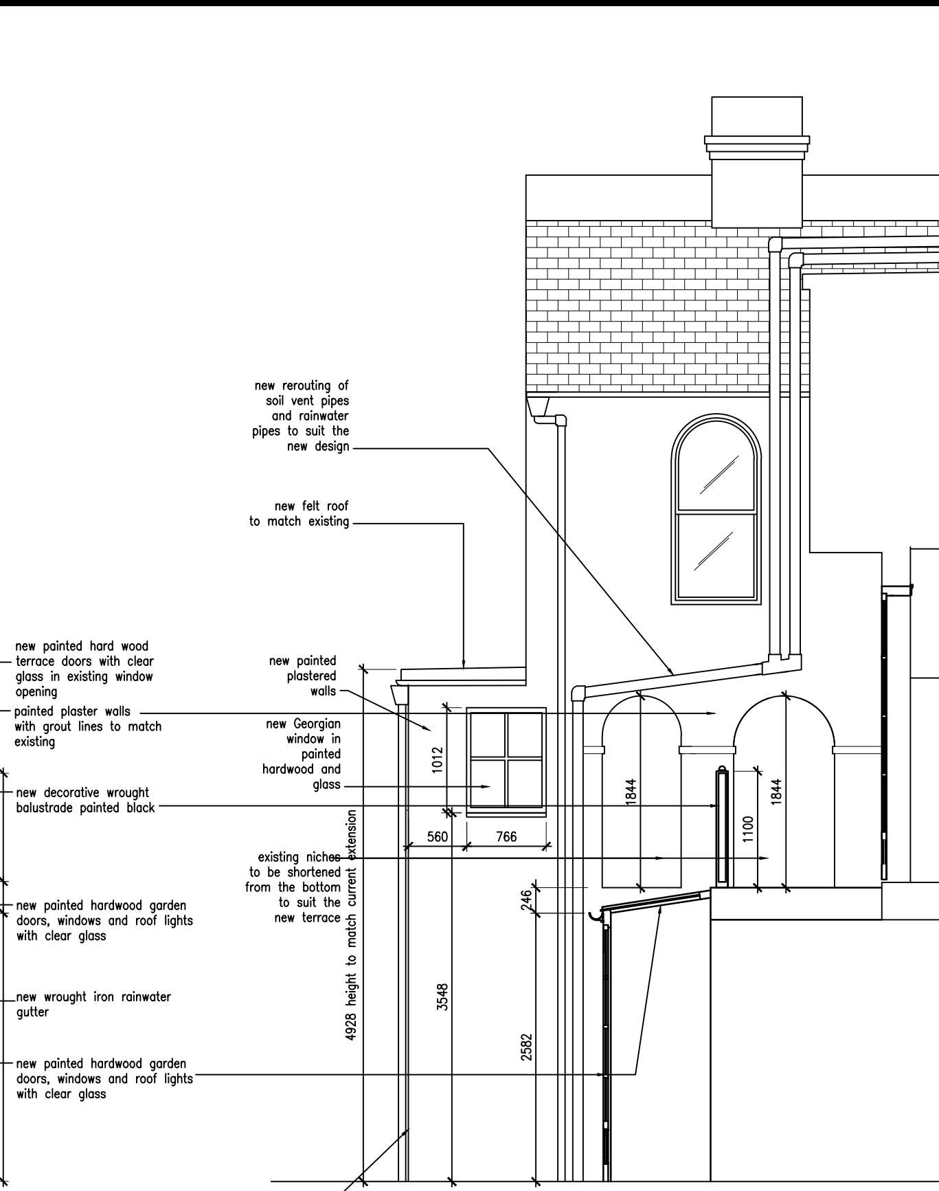
3 Proposed Terrace Door Scale: 1:20@ A3
