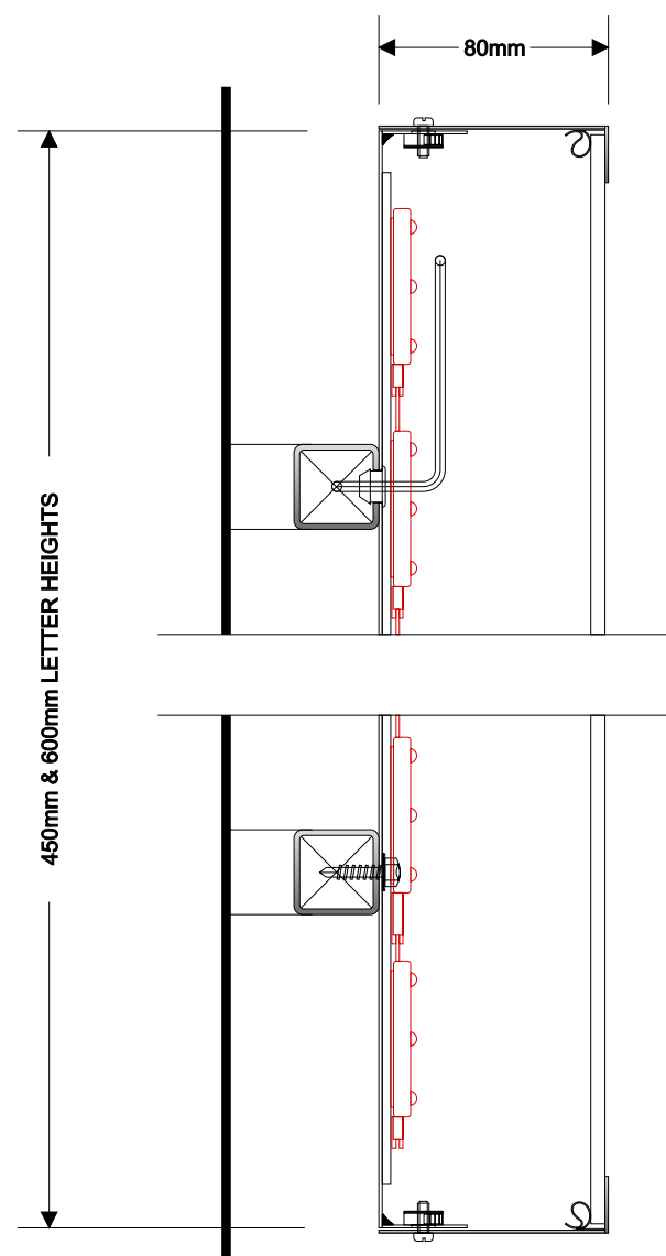
PART SECTION THROUGH A-A
