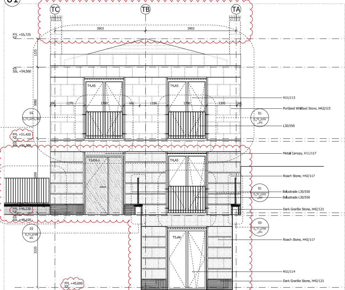
03 NORTH ELEVATION
