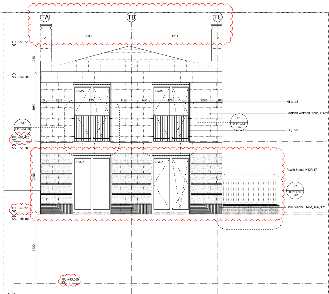
01 SOUTH ELEVATION
