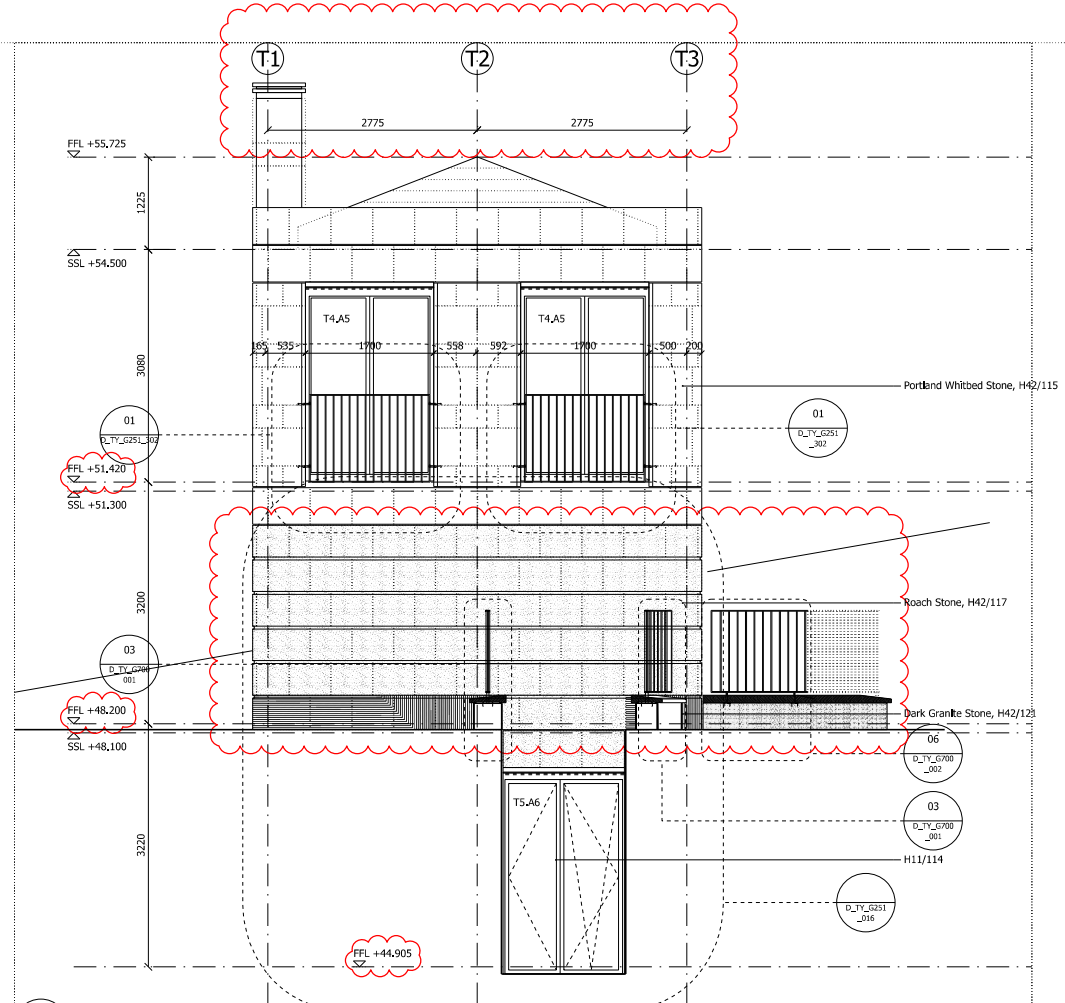
02 EAST ELEVATION
