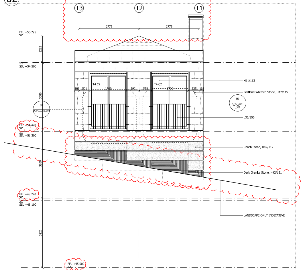
04 WEST ELEVATION
