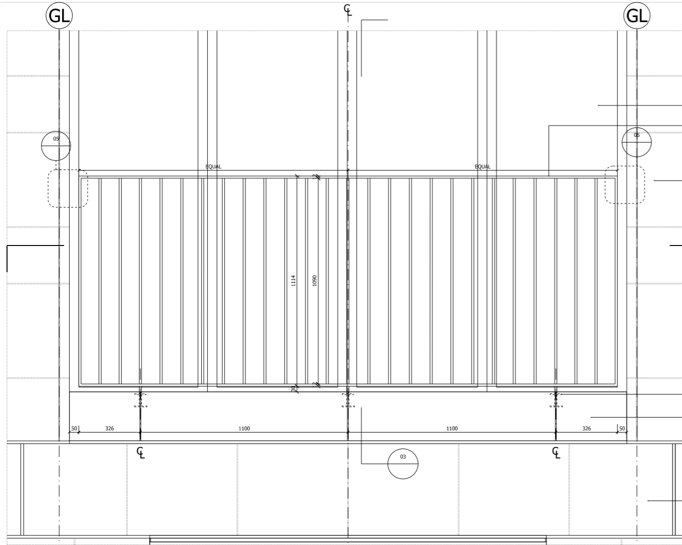
01 TYPICAL ELEVATION DETAIL BALUSTRADE D_TY_G251_Balustrade
