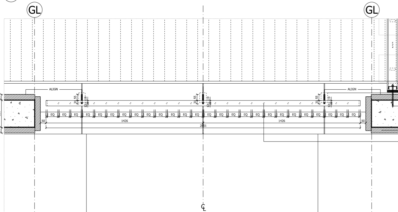
02 TYPICAL PLAN DETAIL BALUSTRADE D_TY_G251_Balustrade
