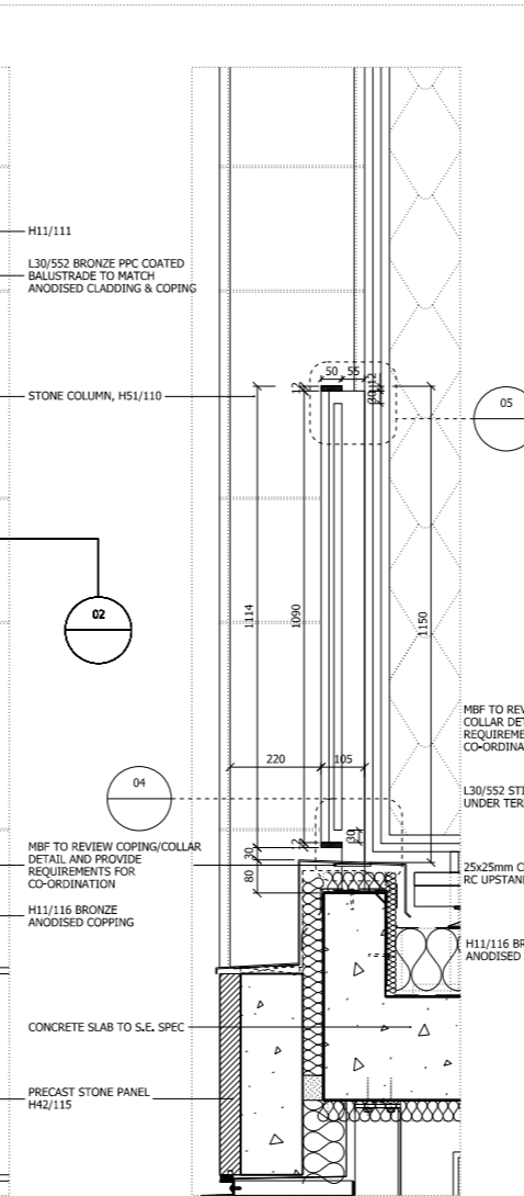
03 TYP. SECTION DETAIL BALUSTR. D_TY_G251_Balustrade
