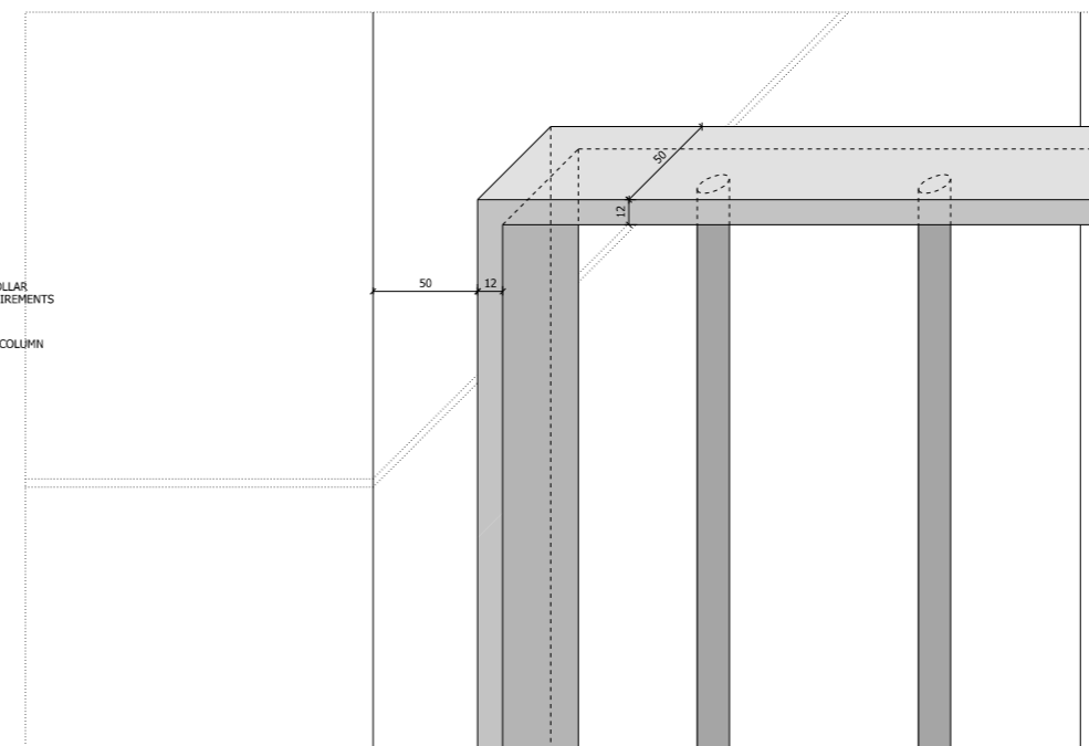
05 TYPICAL DETAIL (1:5) D_TY_G251_Balustrade
