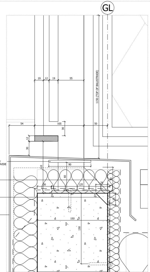
04 TYPICAL DETAIL - FIXING TO CONCRETE (1:5) D_TY_G251_Balustrade
