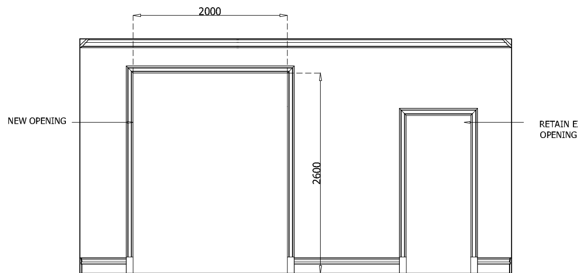
PROPOSED ELEVATION D
