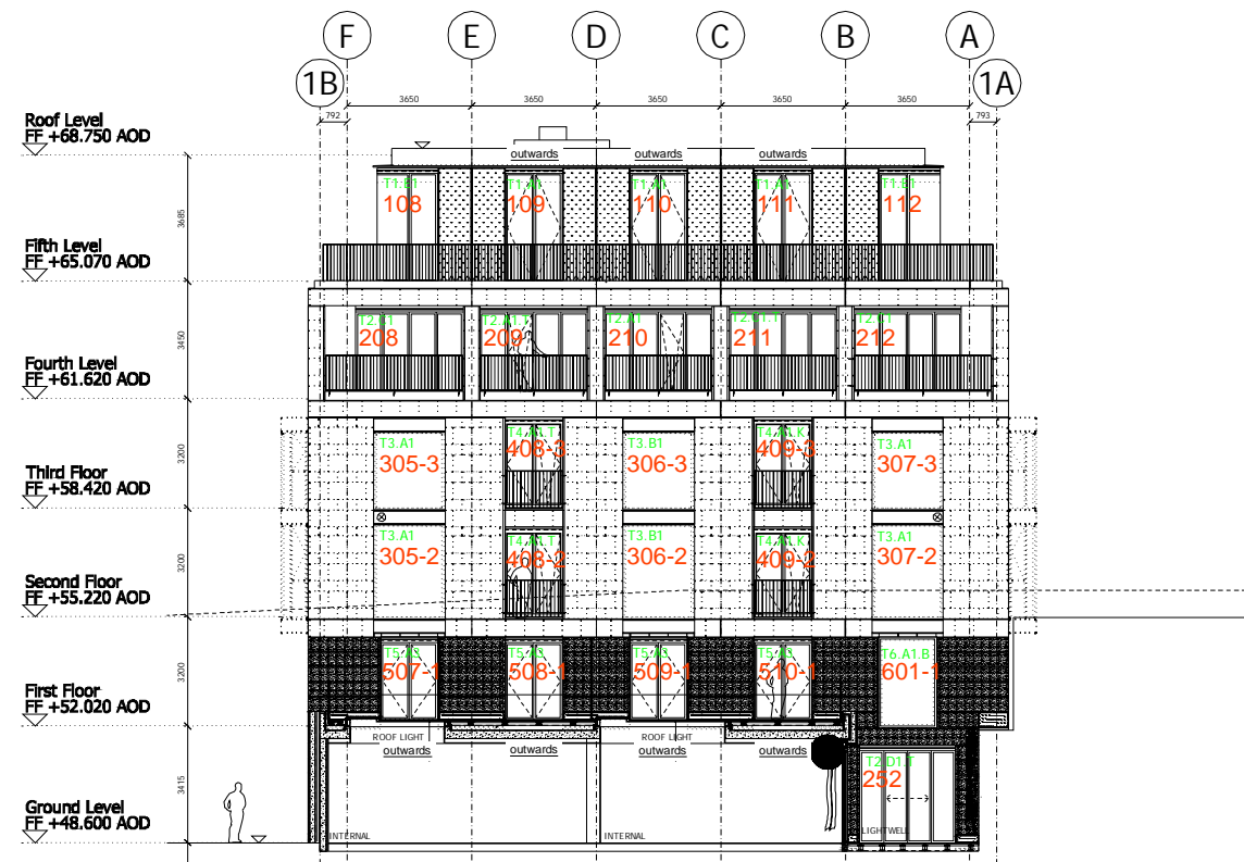
Block 1 North Elevation
