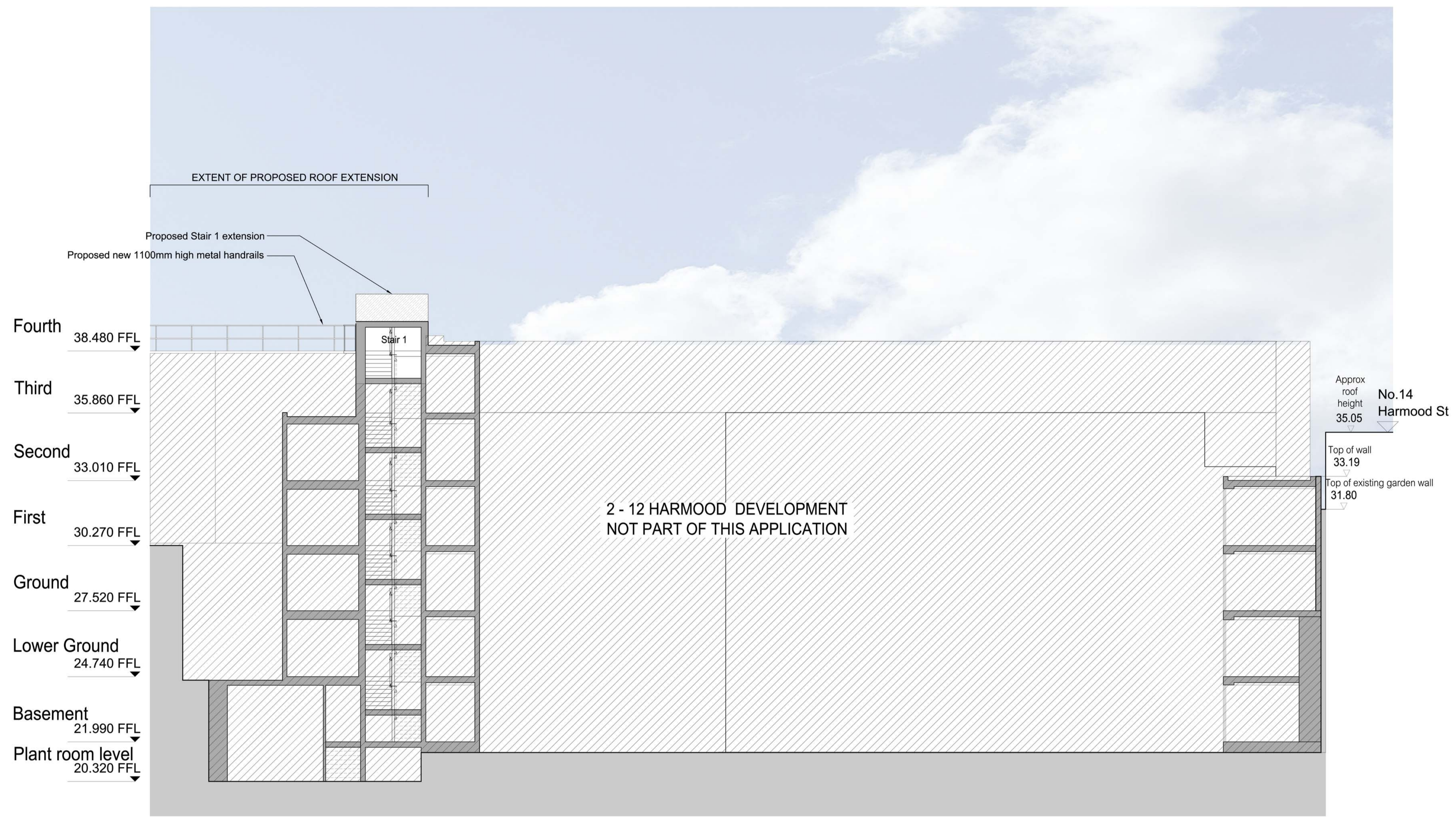
PROPOSED SECTION BB'
