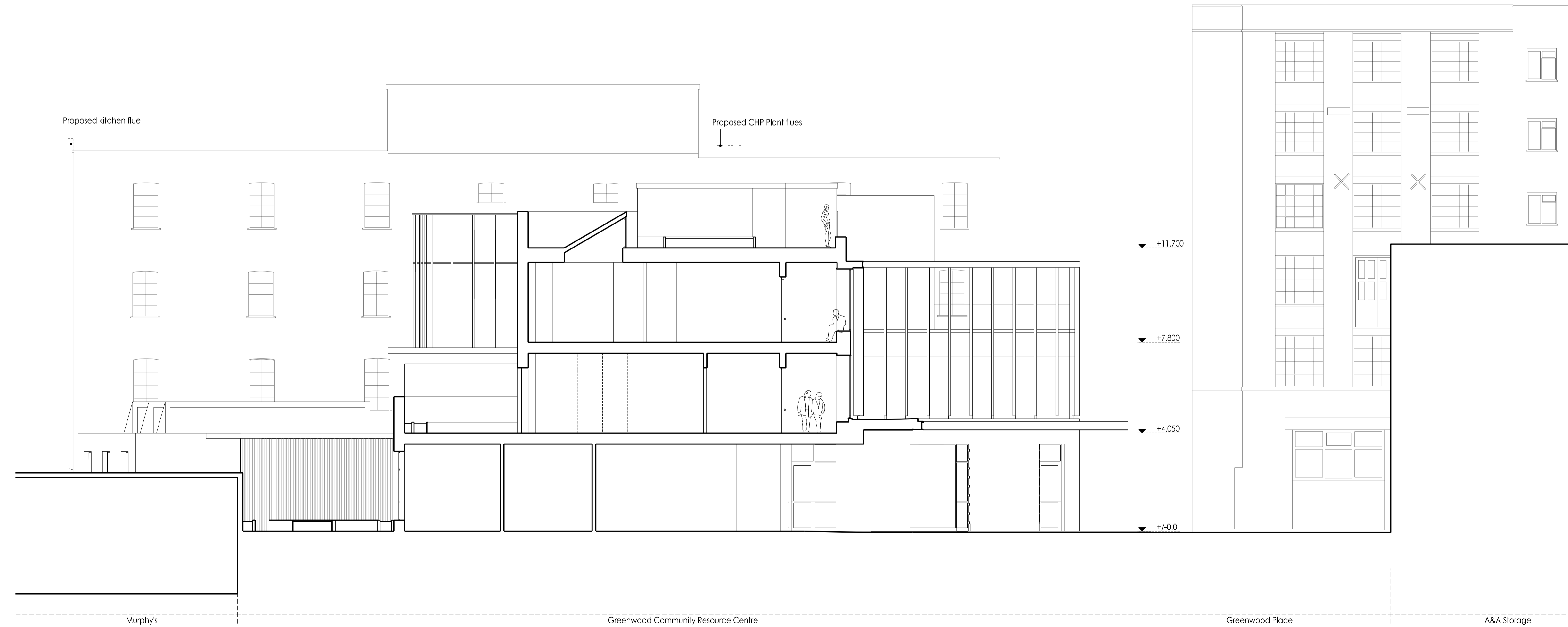
SECTION B-B
