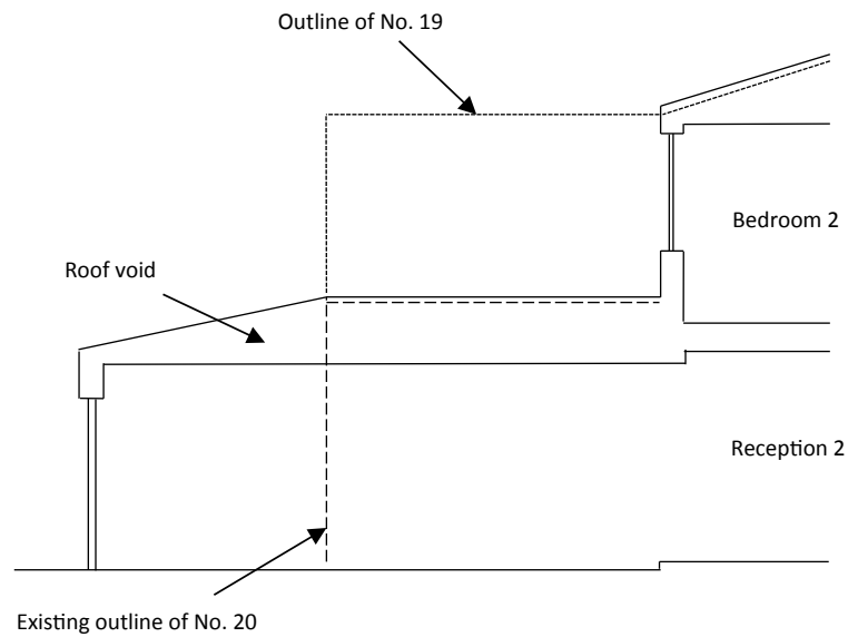
Proposed East Elevation (Section C-C)
