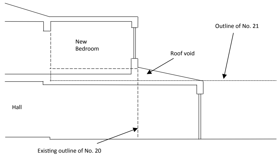
Proposed West Elevation (Section D-D)
