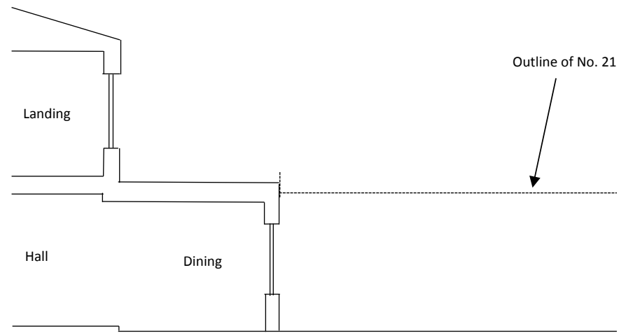
Proposed West Elevation (Section B-B)
