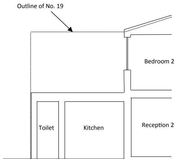
Existing East Elevation (Section A-A)
