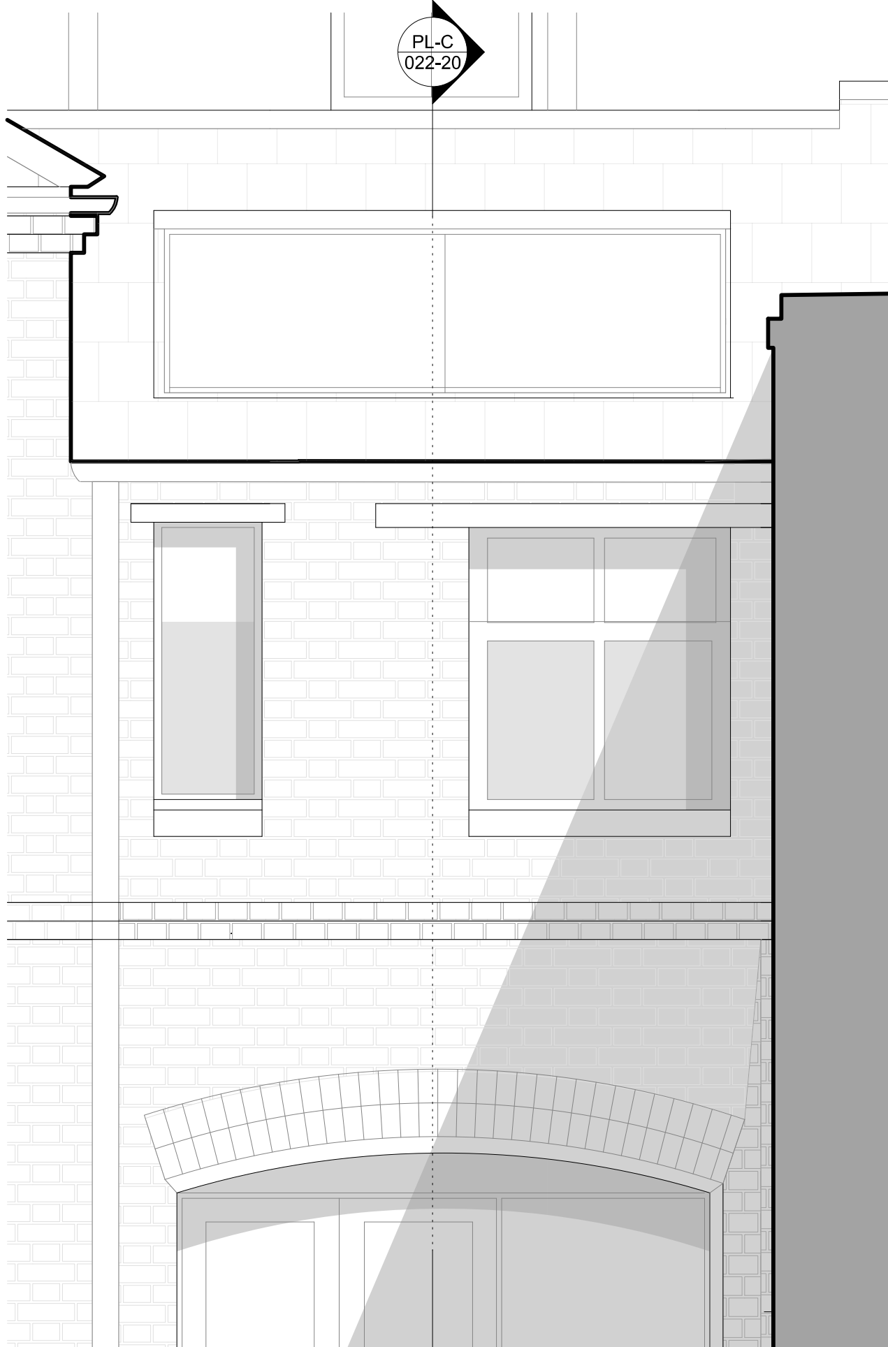
PL-B 022-20 Endell Street Proposed skylight detail 1:50
