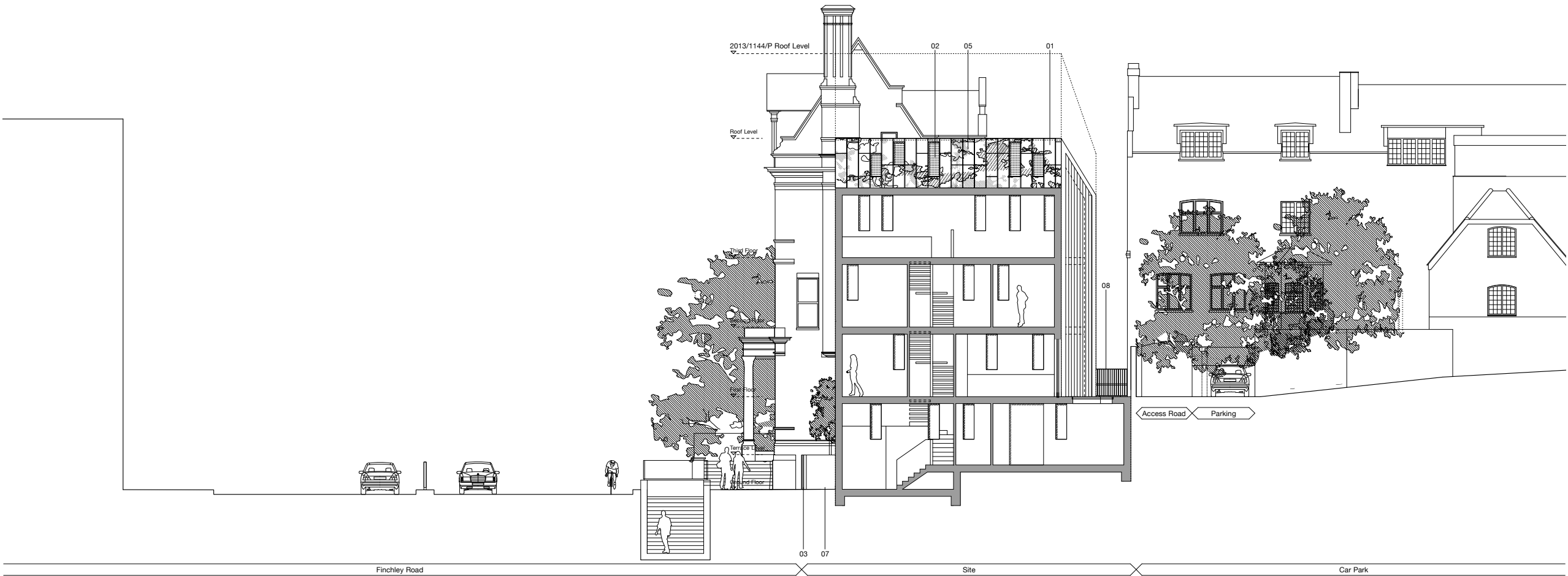
01 SOUTH EAST ELEVATION Scale : 1:100
