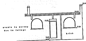
GARAGE AND WORKSHOP ELEVATION
