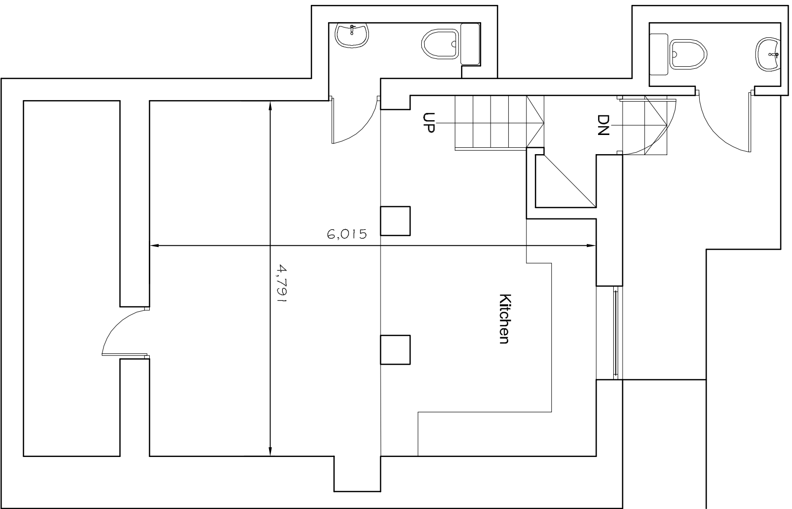
EXISTING BASEMENT FLOOR PLAN
