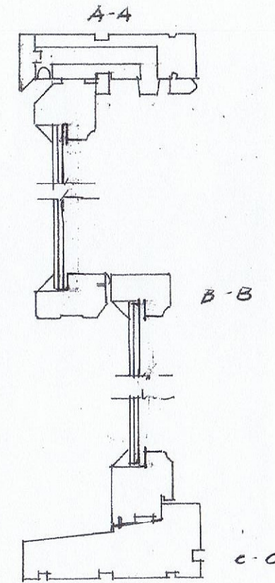
SECTION 1-5
