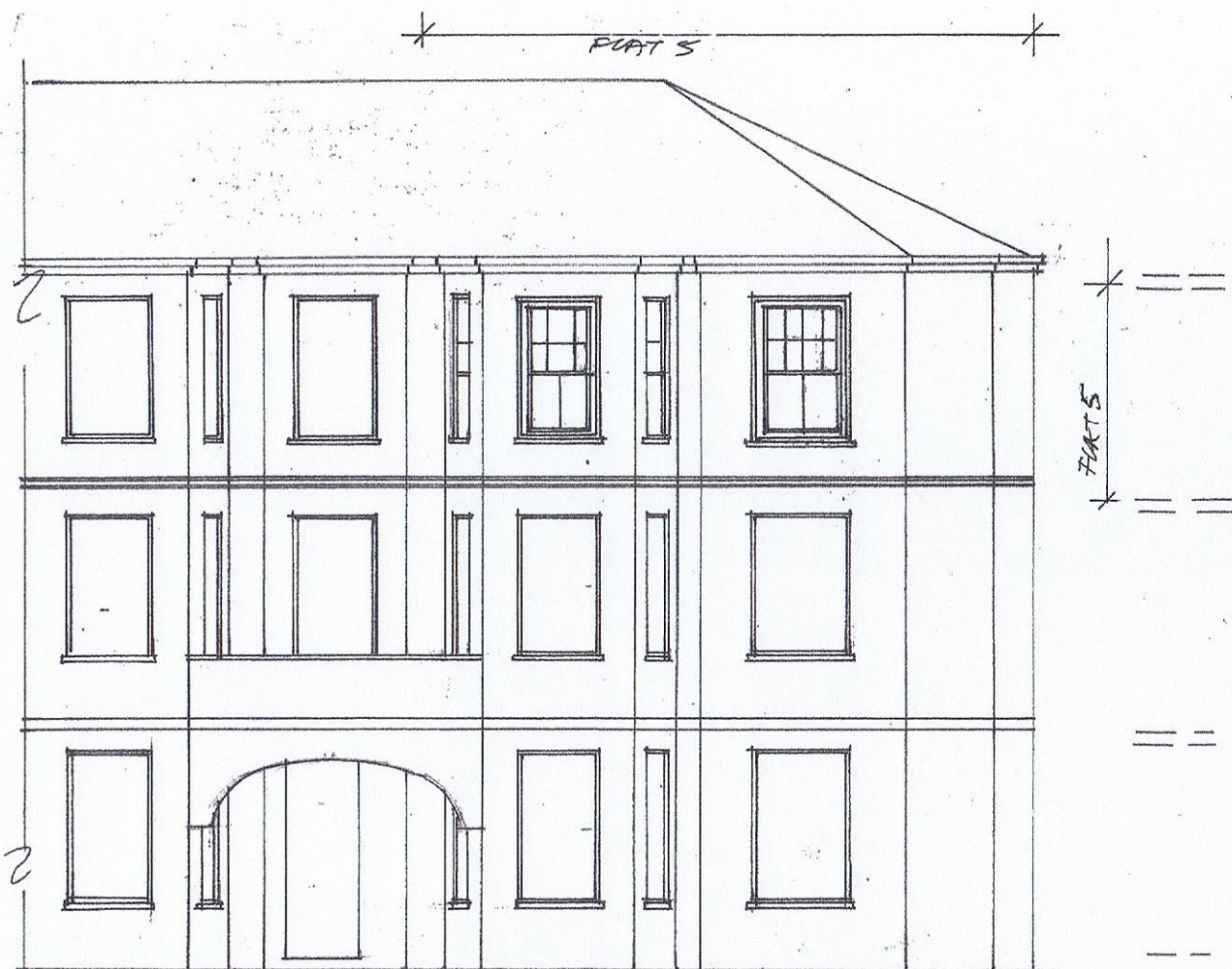
FRONT ELEVATION
