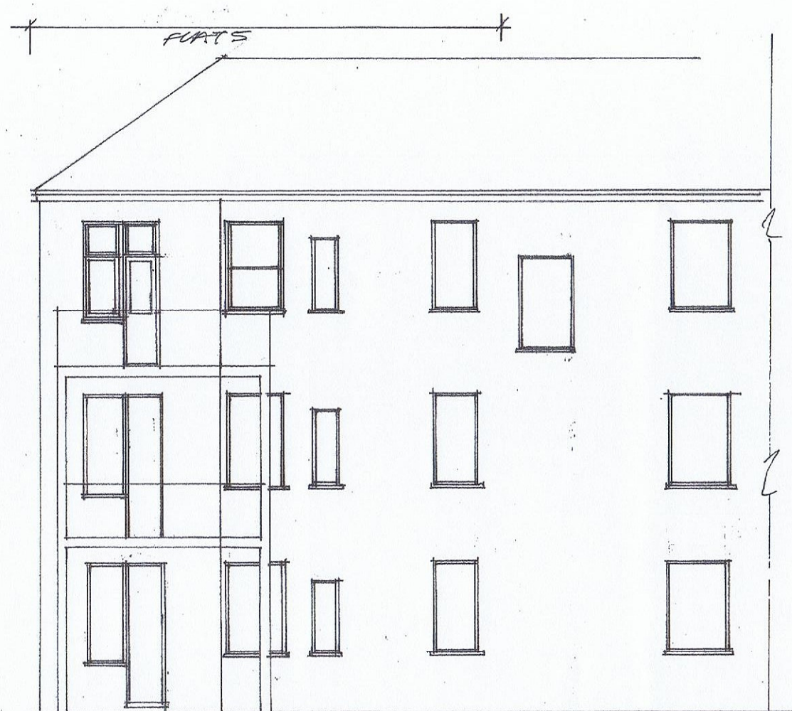
REAR ELEVATION
