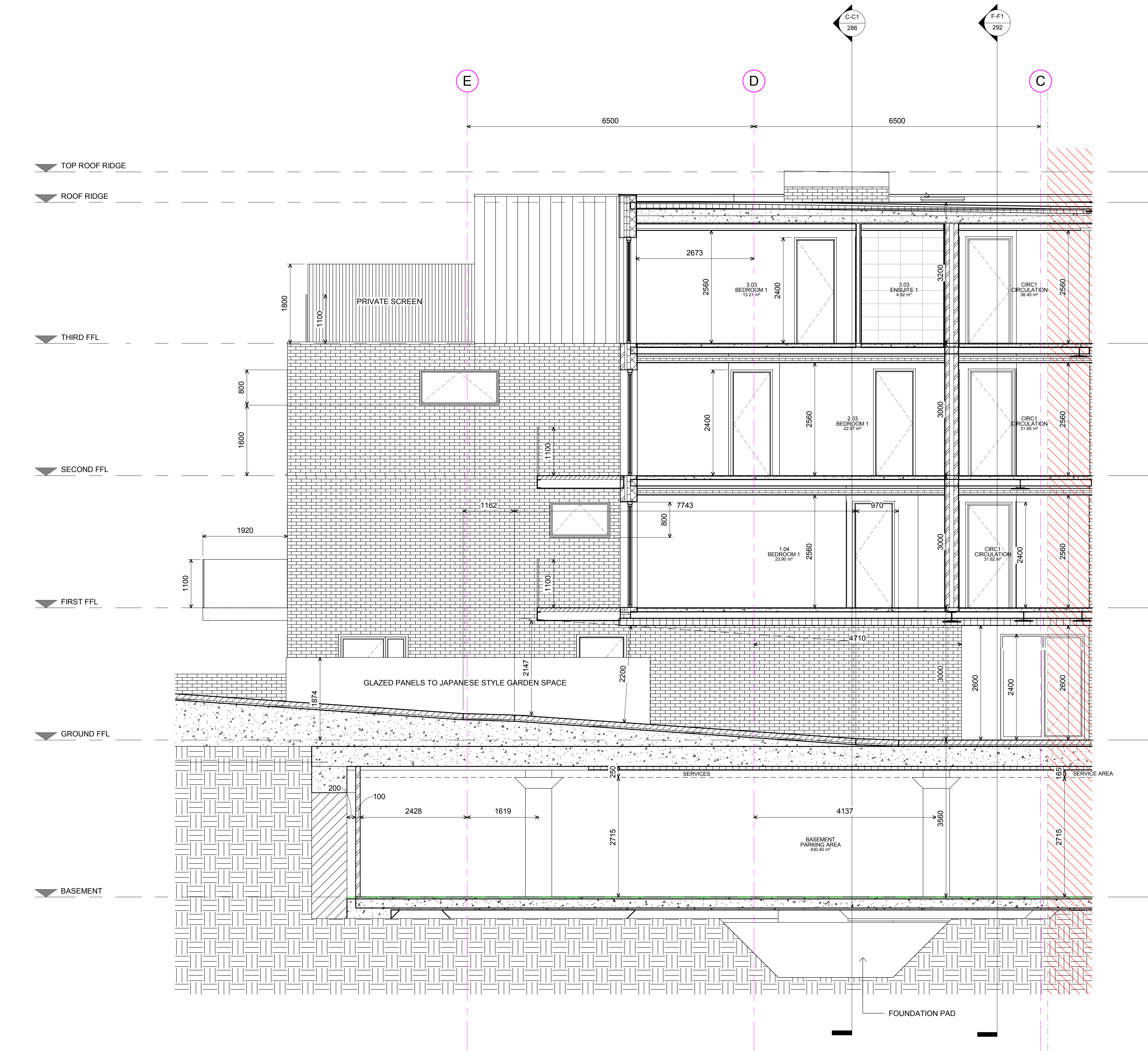
E-E1 SECTION E-E - Sheet 1
