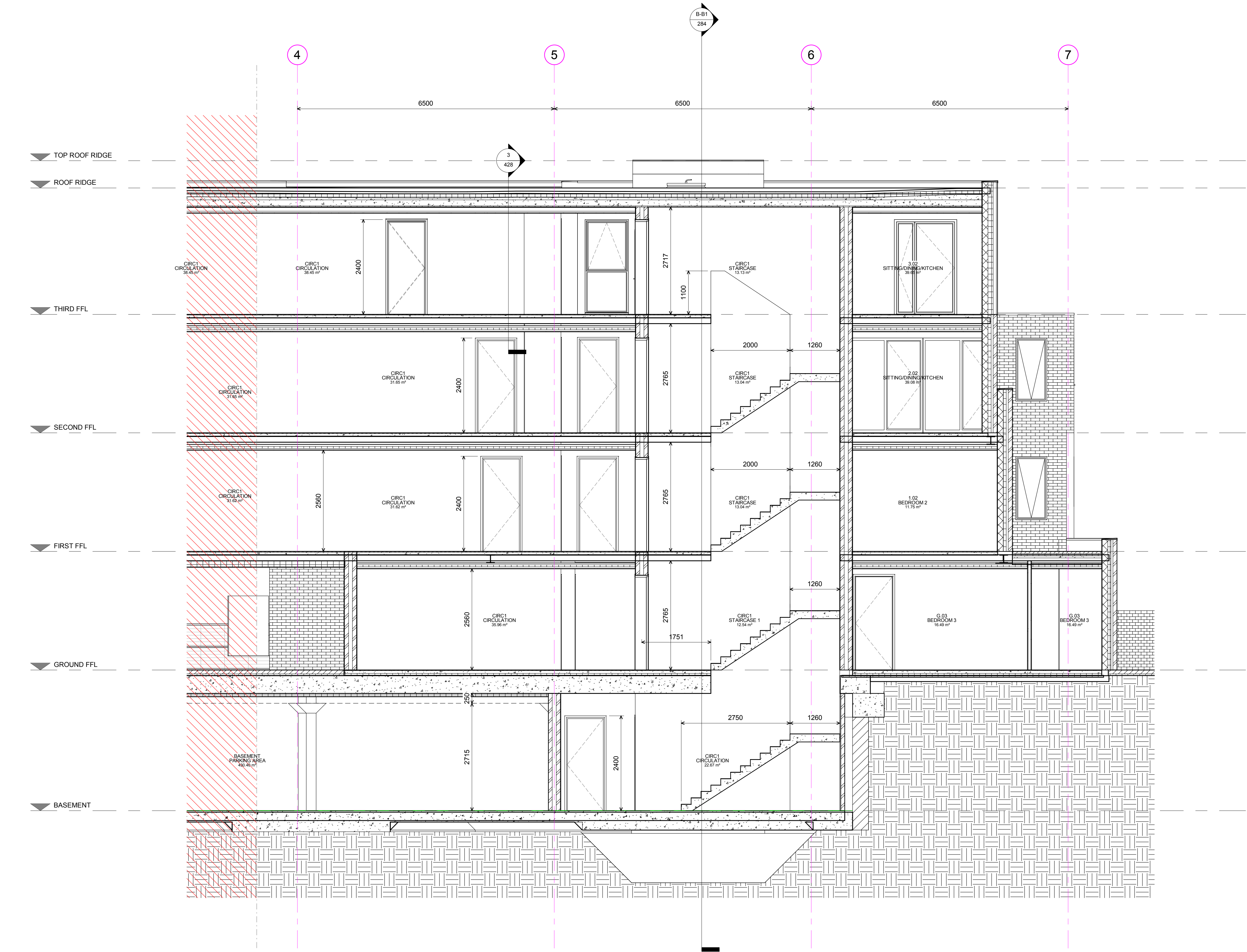
SECTION F-F - Sheet 2
