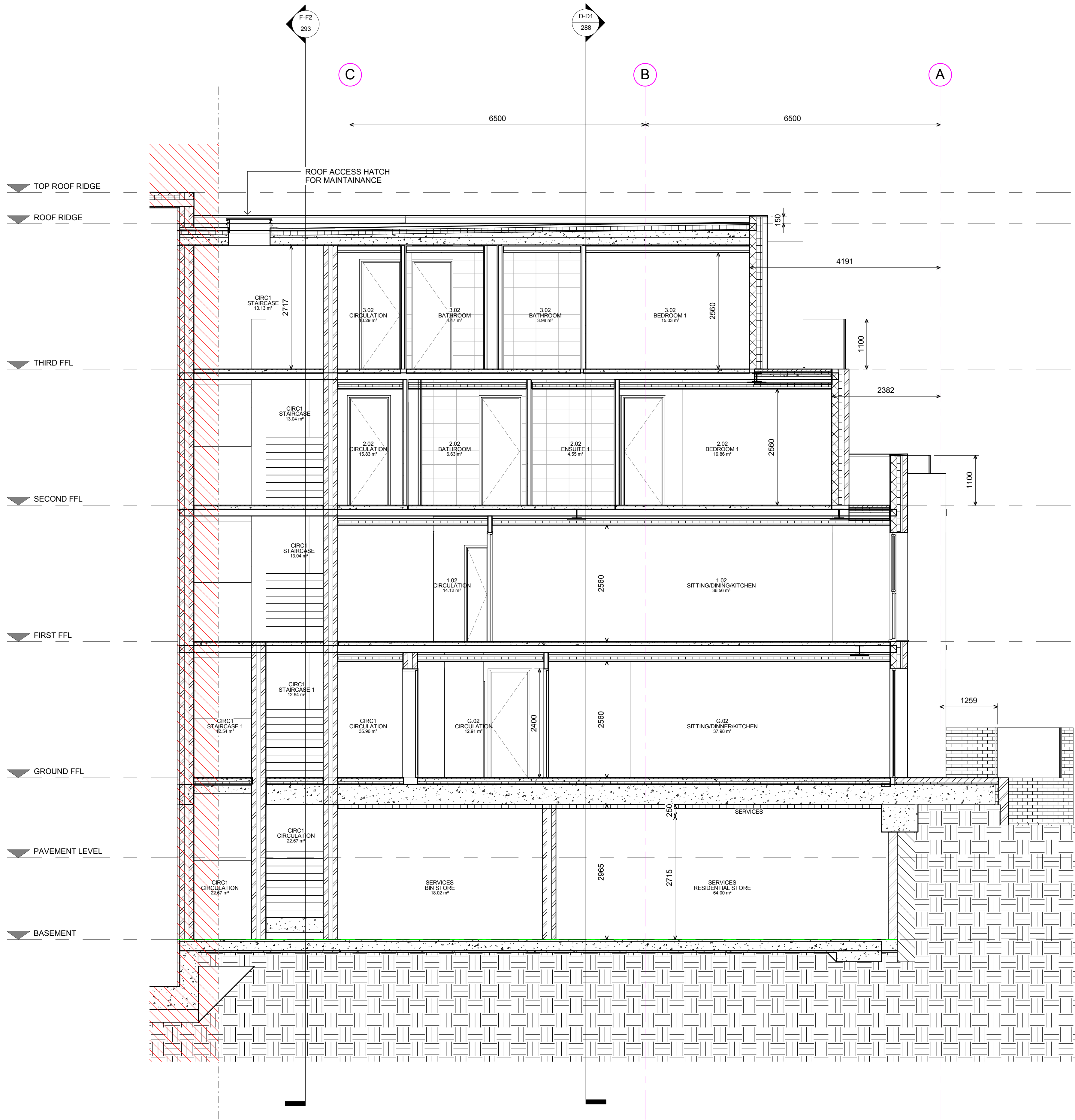
B-B2 SECTION B-B - Sheet 2
