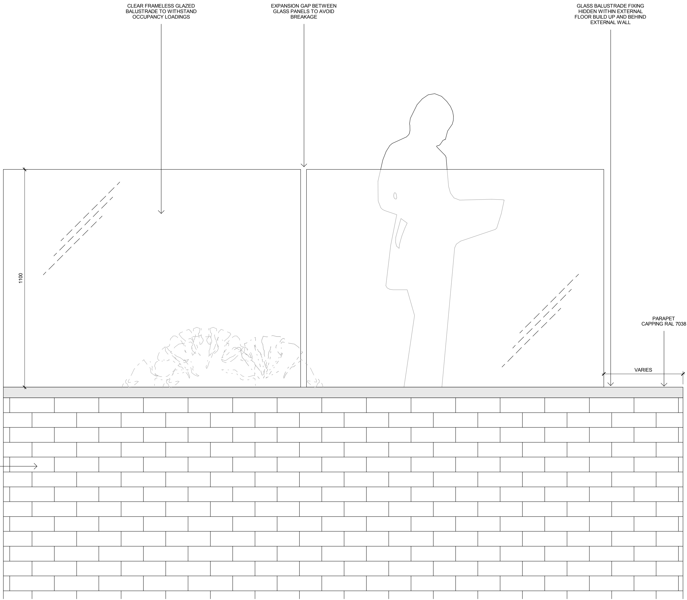
TYPICAL BALUSTRADE ELEVATION 1:10
