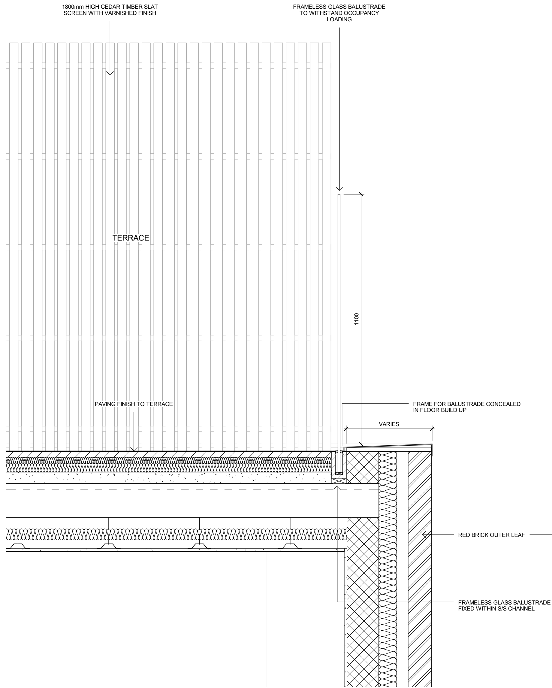
TYPICAL BALUSTRADE DETAIL 1:10
