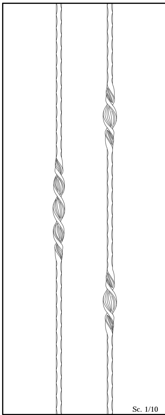
Details of the proposed balustrades.
