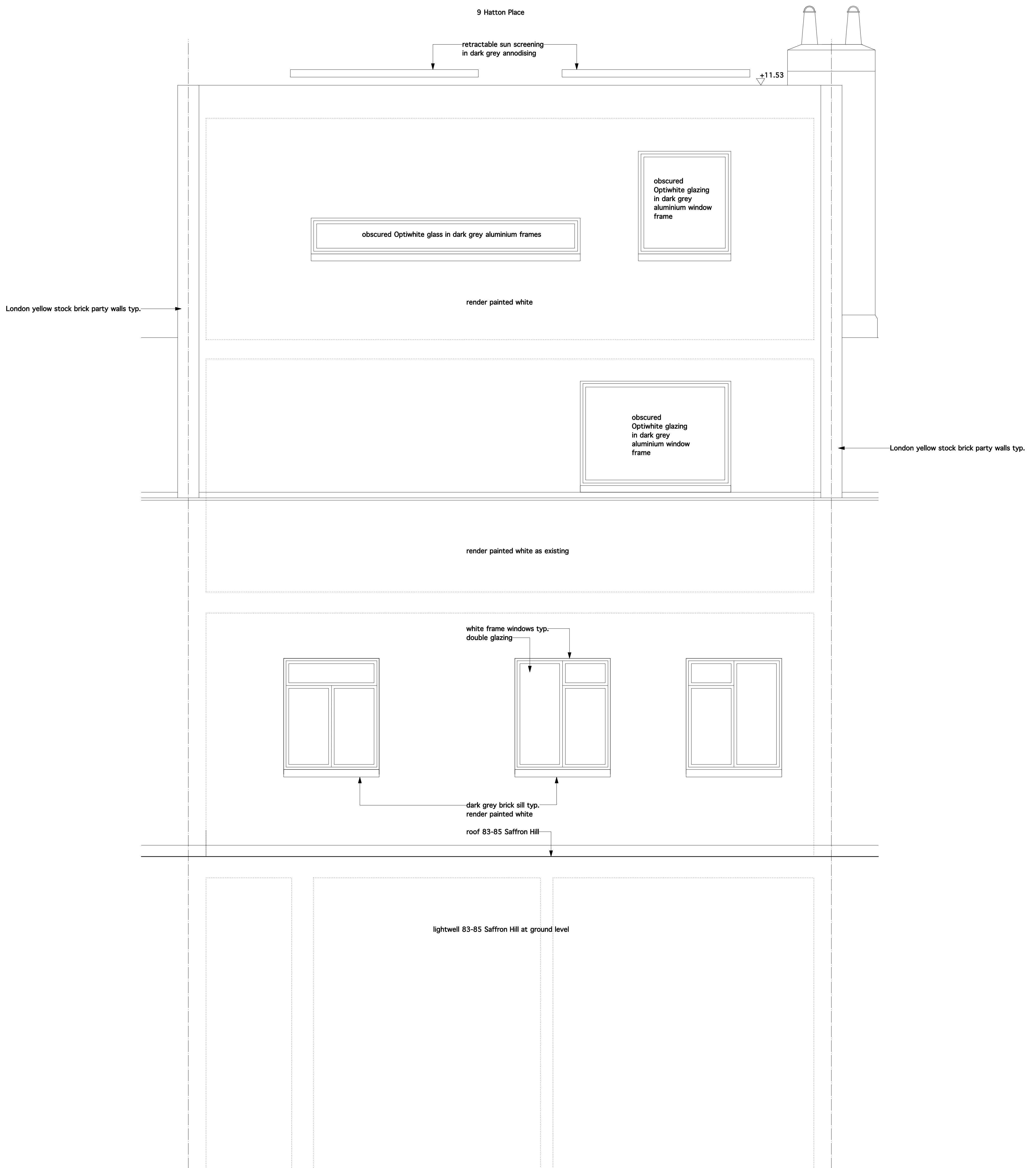
proposed 9 Hatton Place rear elevation 1:20
