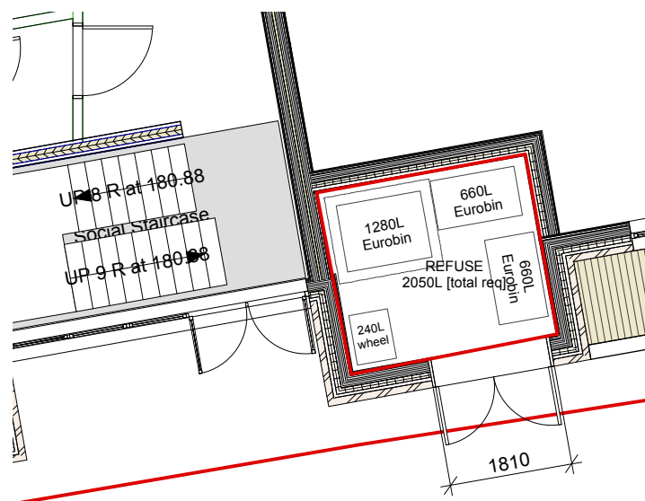
Refuse Storage Location - Social Block 11 m 2
