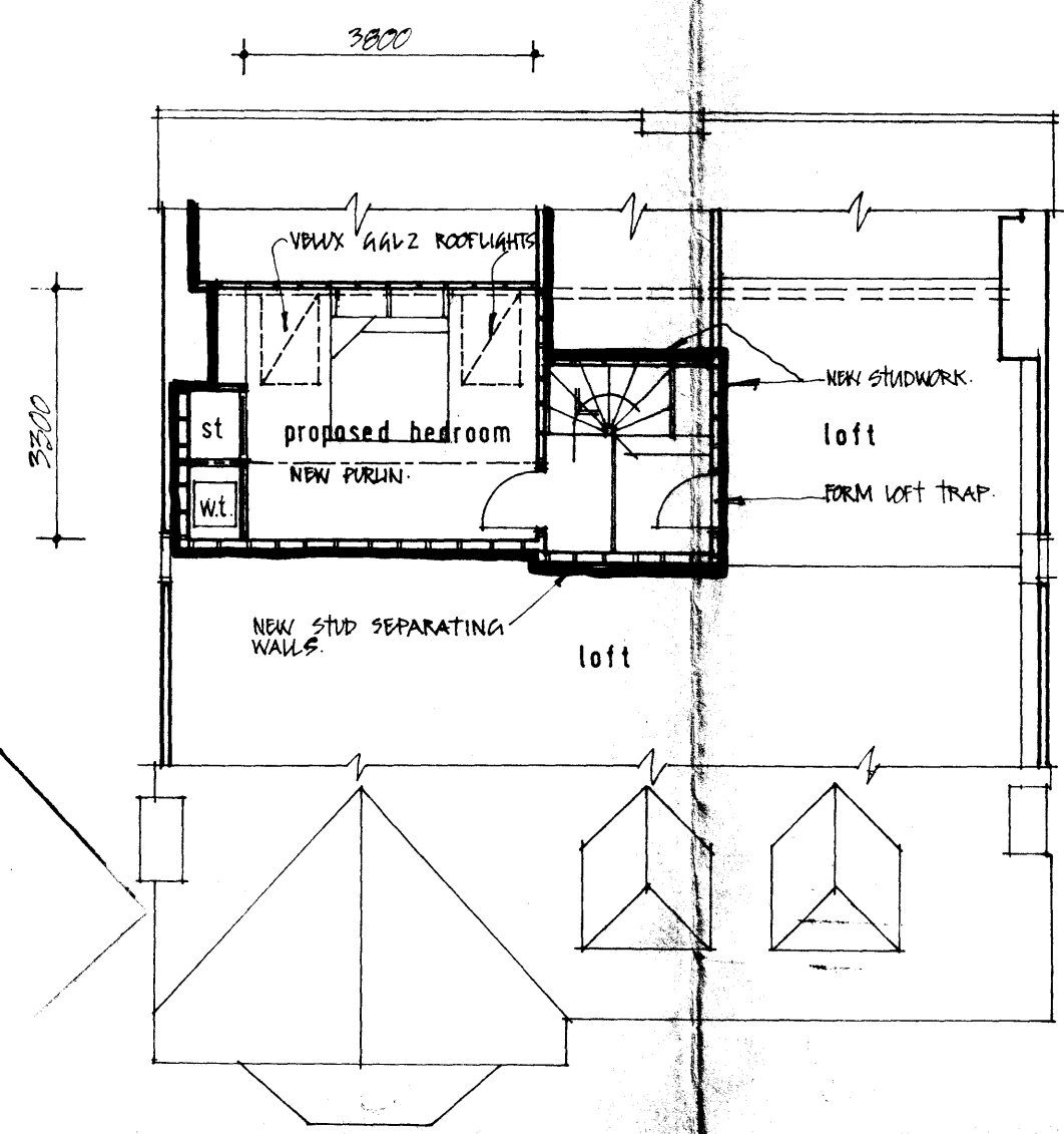
ATTIC / ROOF LEVEL
