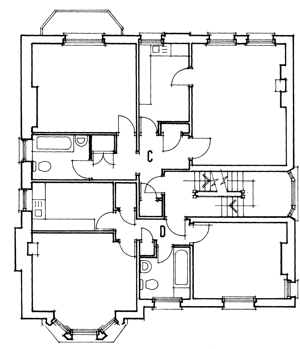
FIRST FLOOR
