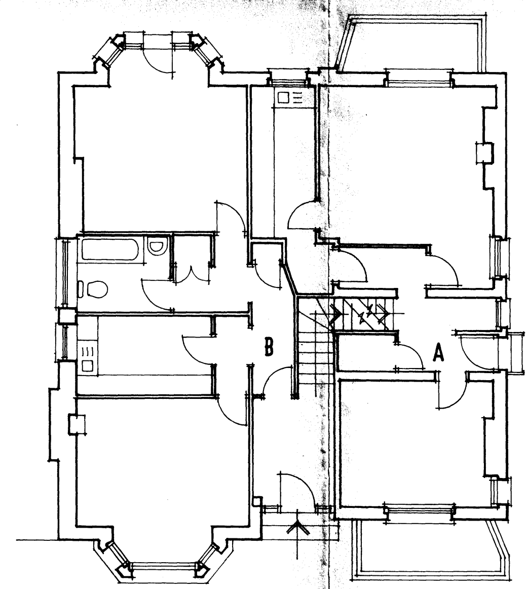
GROUND FLOOR
