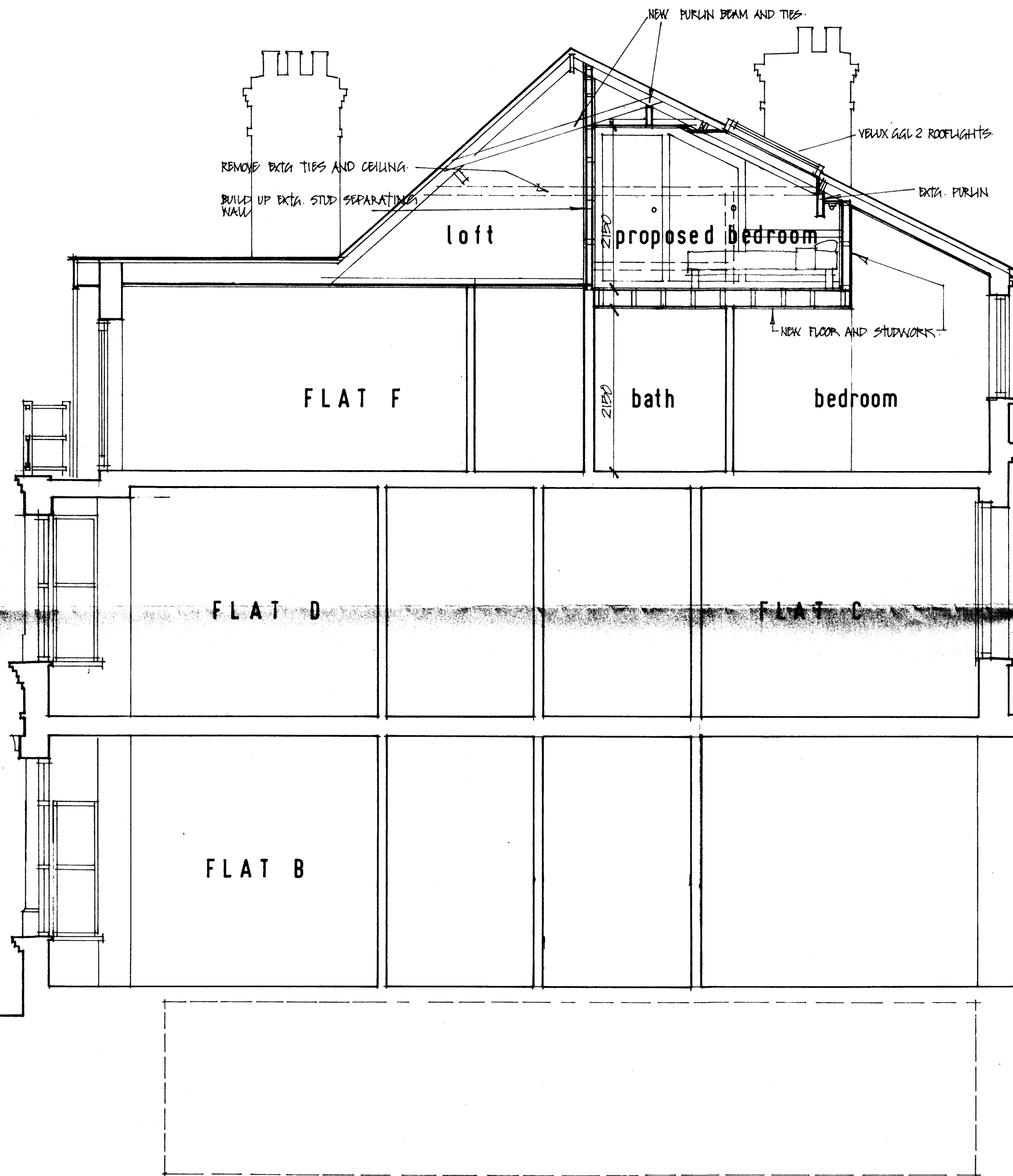
SECTION 1:50
