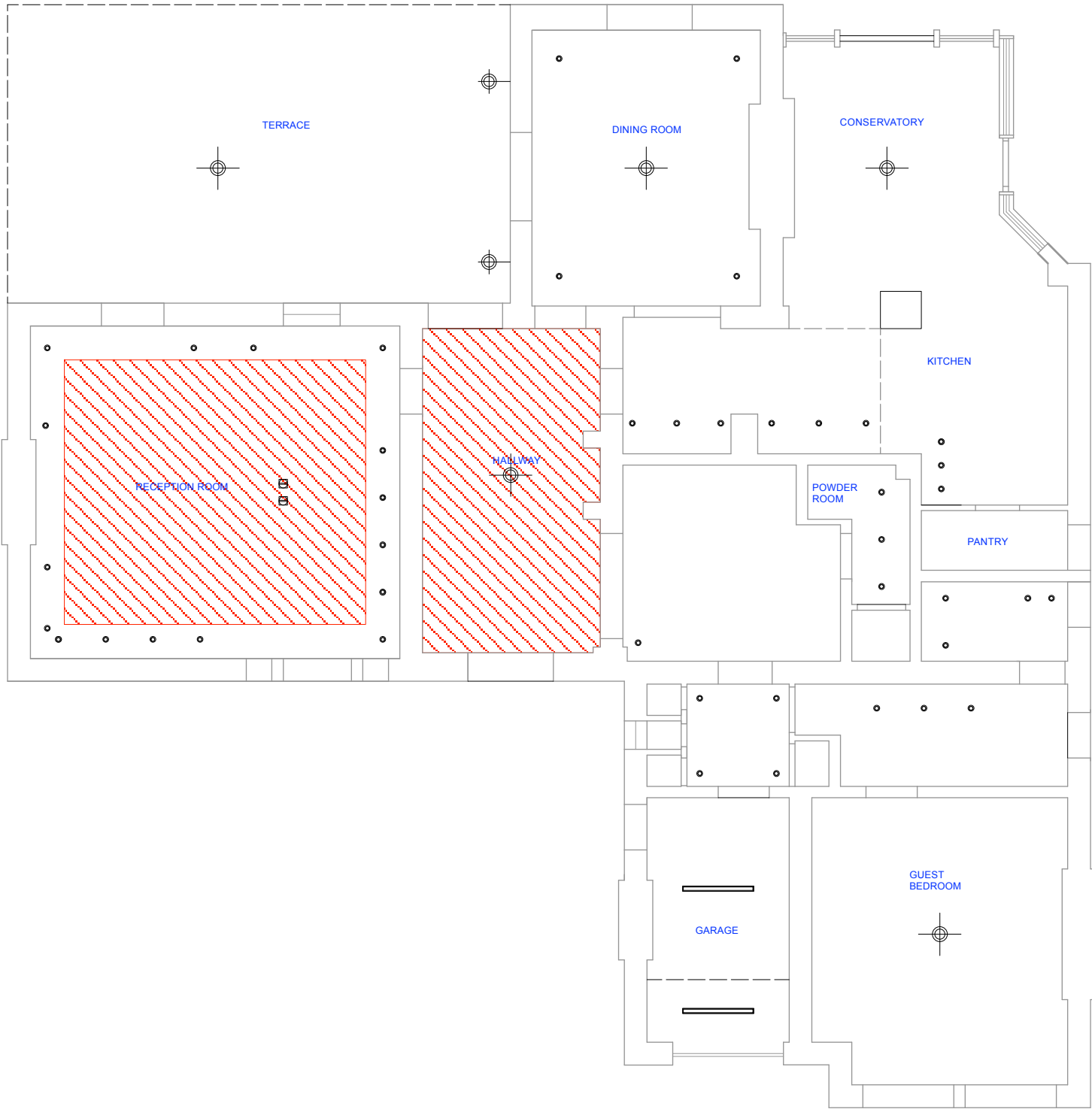
1 REFLECTIVE CEILING PLAN Scale: 1:100
