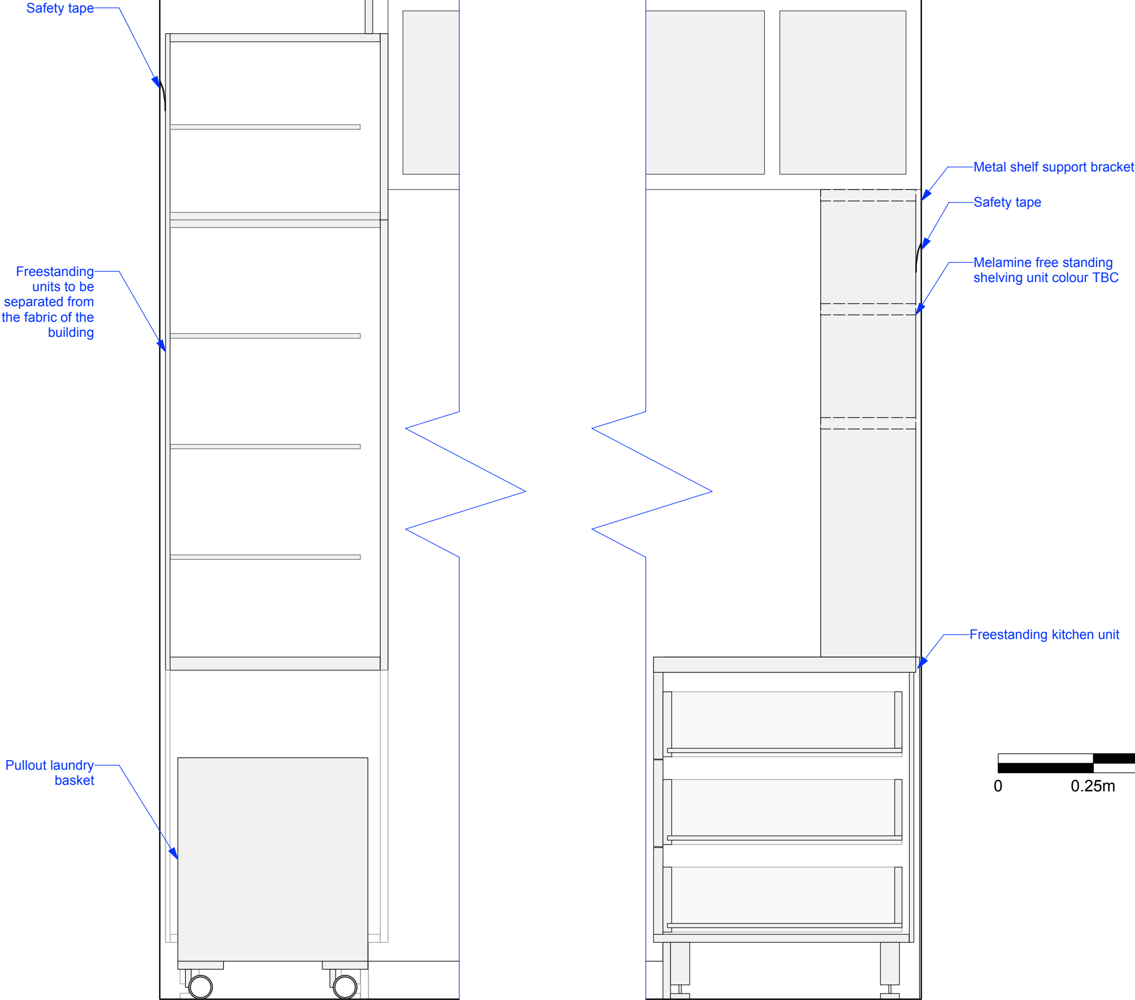
1 DETAILED SECTION Scale: 1:10
