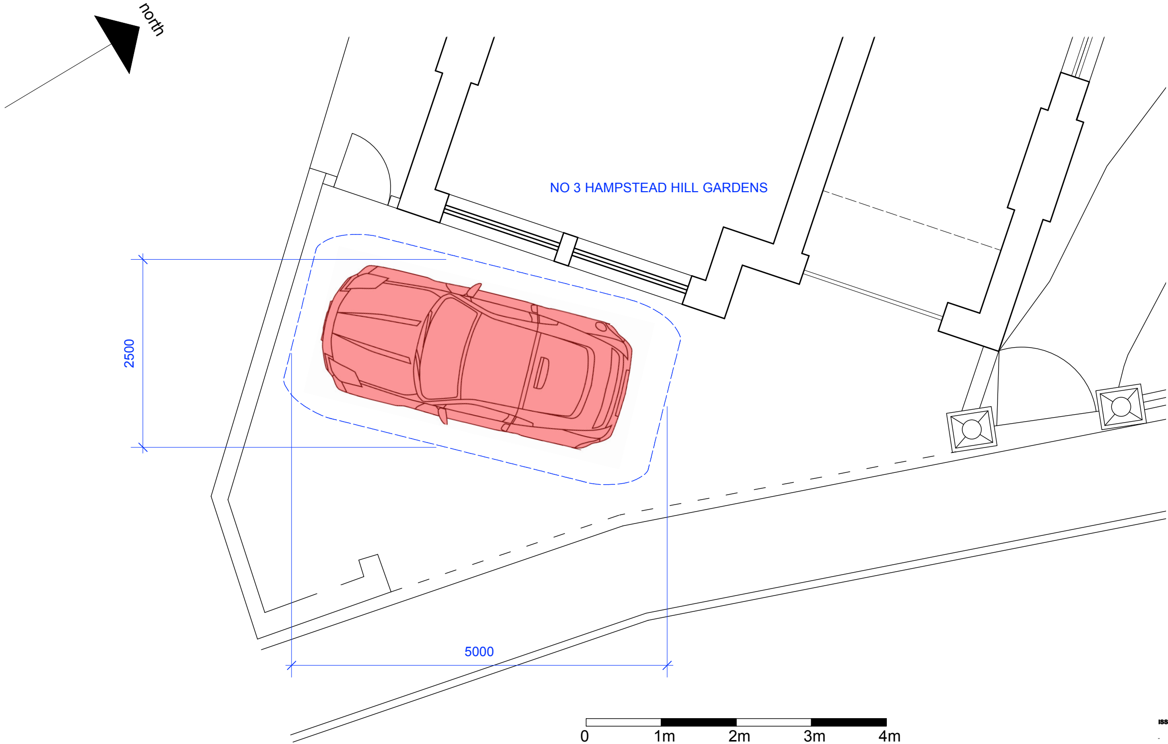
1 PARKING AREA Scale: 1:50
